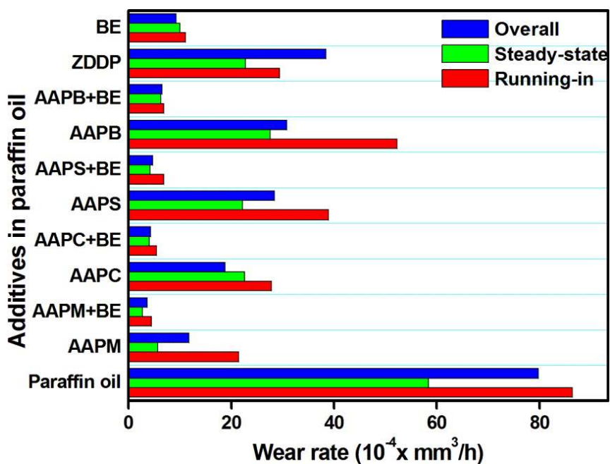
Figure 3.5. Wear-rates for paraffin oil in the presence and absence of different additives and their synergistic formulations (1%w/v) at 392N applied load for 90 min test duration
