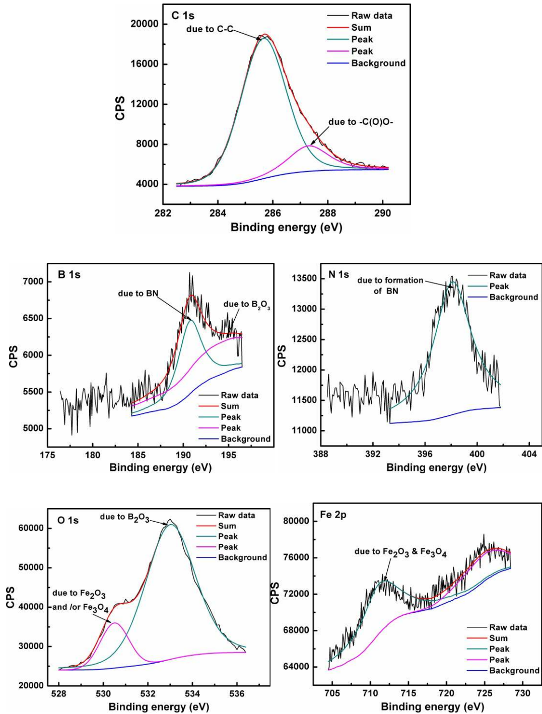
Figure 3.12. XPS spectra of tribochemical film formed on worn steel surface lubricated with AAPM+BE (1% w/v) at 392N applied load for 90 min test duration in liquid paraffin
