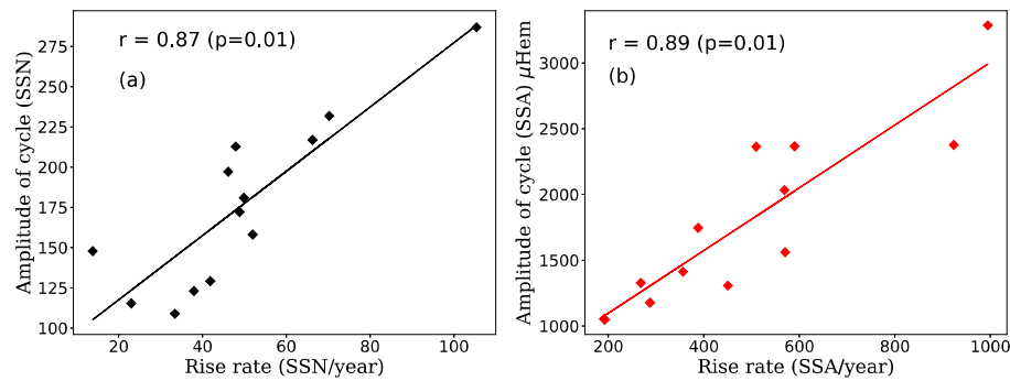
Fig. 4.1 Scatter plots between the rise rates and the amplitudes of the cycles for SSN (a) and SSA (b). Lines are the linear regressions: y = mx + c , where m = 2.001 \pm 0.308 and c = 77.305 \pm 16.545 for SSN and m = 2.423 \pm 0.114 and c = 596.789 \pm 62.028 for SSA.
