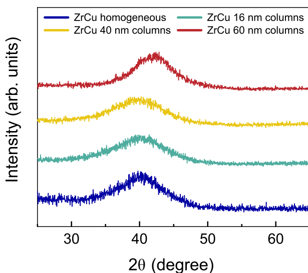
Fig. 2. XRD patterns of homogeneous and nanocolumnar ZrCu TFMGs showing a fully amorphous structure.
