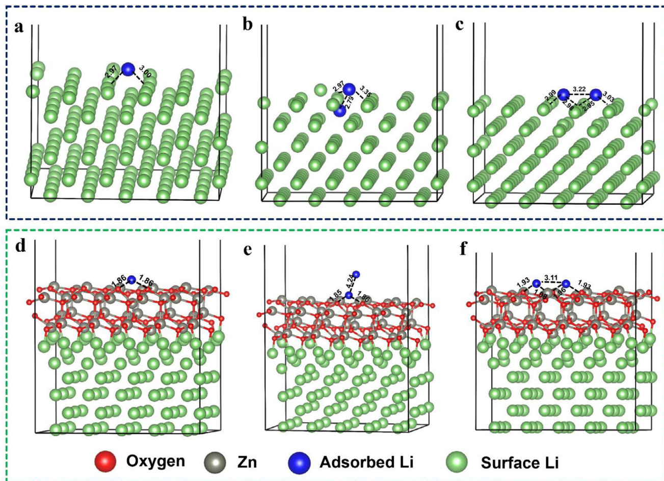
Figure 6. Optimized structures of a) Li (100) and d) Li(100)/ZnO after the adsorption of the first Li atom. Optimized structures of b,c) Li(100) and e,f) Li(100)/ZnO after the “on-top” (b,e) and (c,f) “side-by” adsorption of the second Li atom. Crucial distances (in Å) between the adsorbed Li atom(s) and surface atoms are shown.
