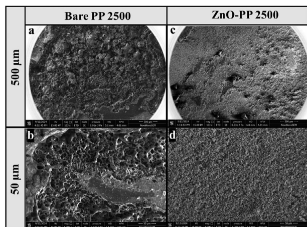
Figure 5. Post-cycling HR-SEM image of a,b) Li-Bare PP c,d) Li-ZnO-PP.
