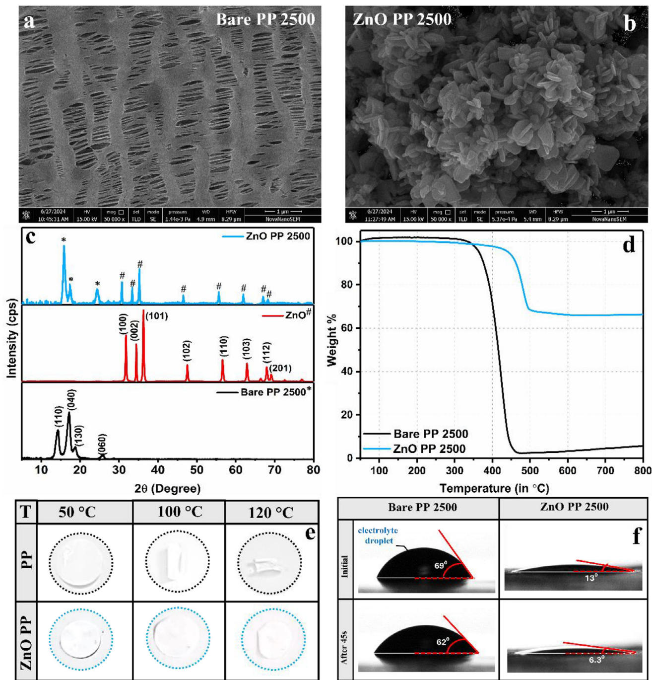
Figure 1. HR-SEM images of a) Bare PP b) ZnO-PP, Comparative c) XRD patterns, d) TGA plots, e) Thermal shrinkage, f) contact angle measurements of Bare and ZnO-PP separator.
