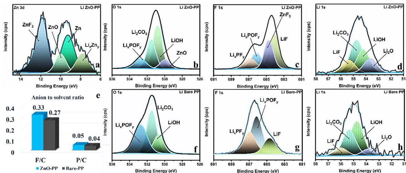
Figure 4. Post-cycling XPS analysis: Deconvoluted a) Zn 3d, b) O 1s, c) F 1s, d) Li 1s for Li-ZnO-PP, e) Comparative chart of anion to solvent ratio, and Deconvoluted f) O 1s, g) F 1s, h) Li 1s for Li-Bare PP.
