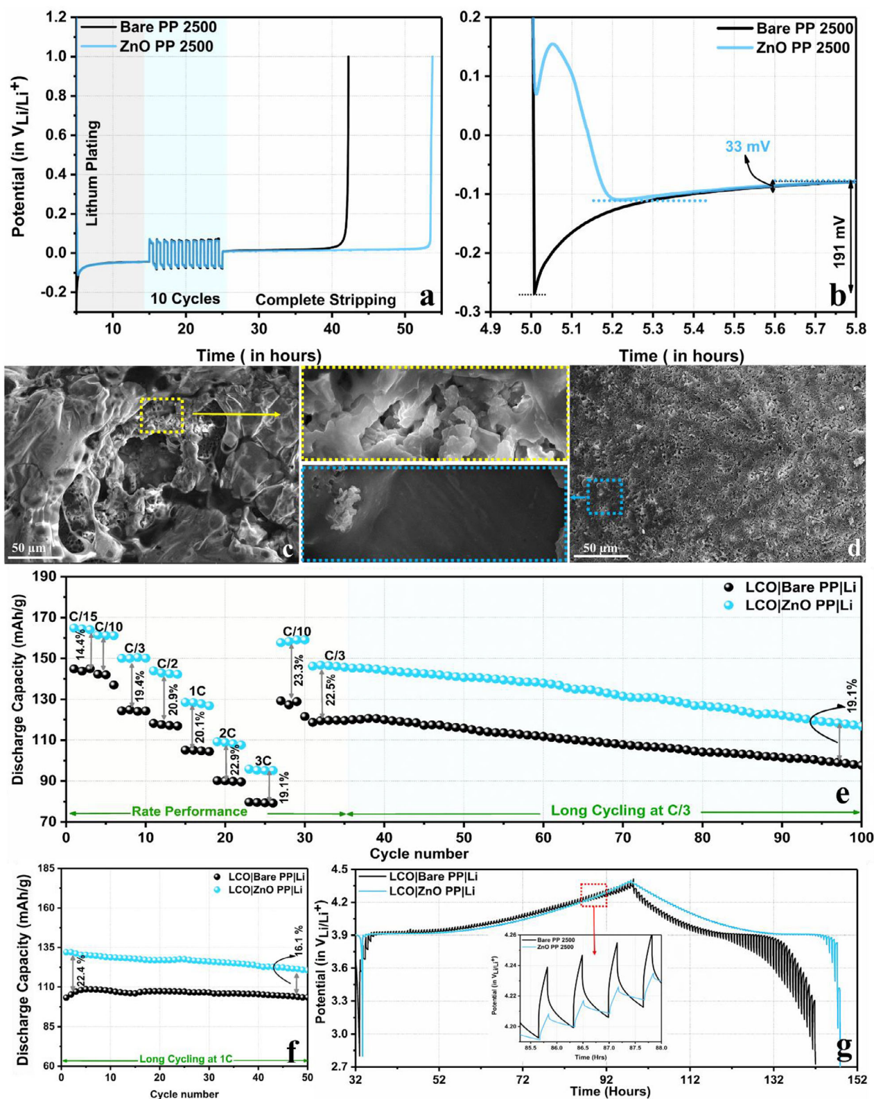
Figure 8. Comparative cycling performance of a) Li|Cu cells, b) observed nucleation overpotentials at Cu current collector. HR-SEM images of Cu current collector after complete lithium stripping in the presence of c) bare PP and d) ZnO-PP separator. Comparative Electrochemical performance of LCO|Bare PP|Li and LCO|ZnO-PP|Li e) under various current densities from C/15 to 3C, and cycling at C/3 and f) 1 C. g) GITT during the charge-discharge cycle at 0.05 C for LCO|Bare PP|Li and LCO|ZnO-PP|Li.
