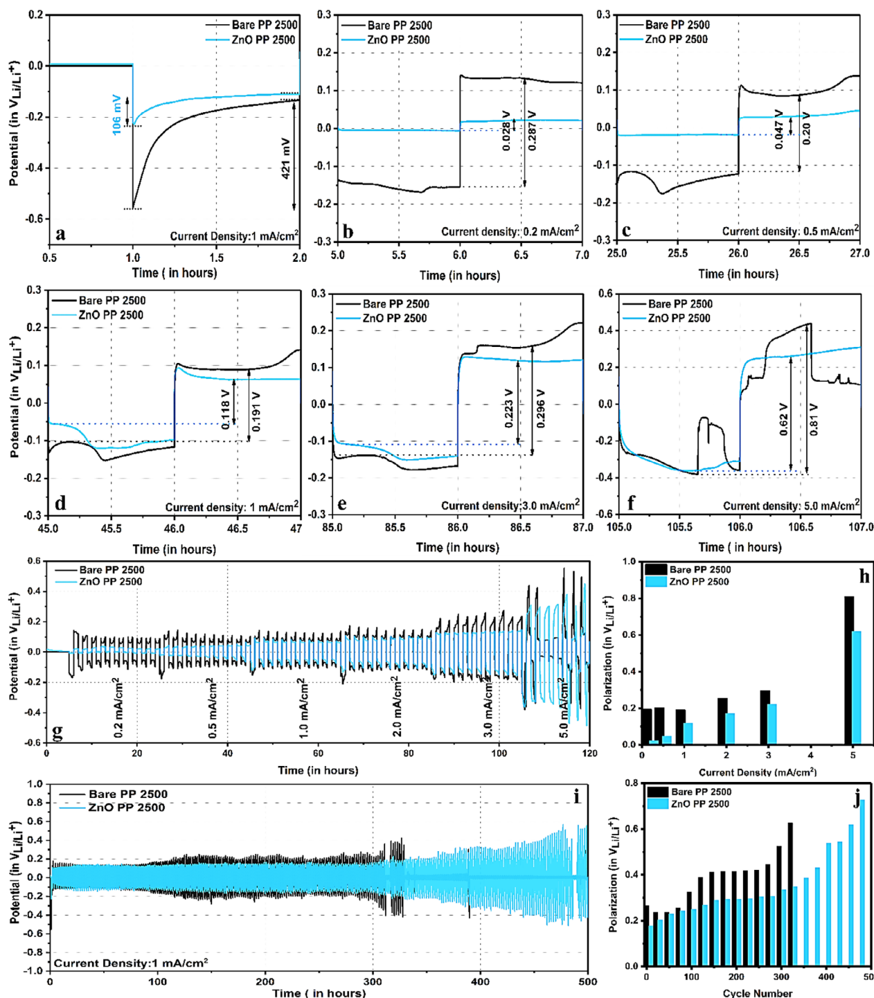
Figure 2. a) Comparative nucleation overpotential at 1 \text{ mA cm}^{-2} . Comparative voltage profiles of Li|Li symmetrical cells at b) 0.2 \text{ mA cm}^{-2} , c) 0.5 \text{ mA cm}^{-2} , d) 1 \text{ mA cm}^{-2} , e) 3 \text{ mA cm}^{-2} , f) 5 \text{ mA cm}^{-2} . Comparative g) Voltage profile and h) corresponding increase in voltage polarization at different current densities. Comparative i) cycling performance and j) corresponding increase in polarization as a function of cycle number.
