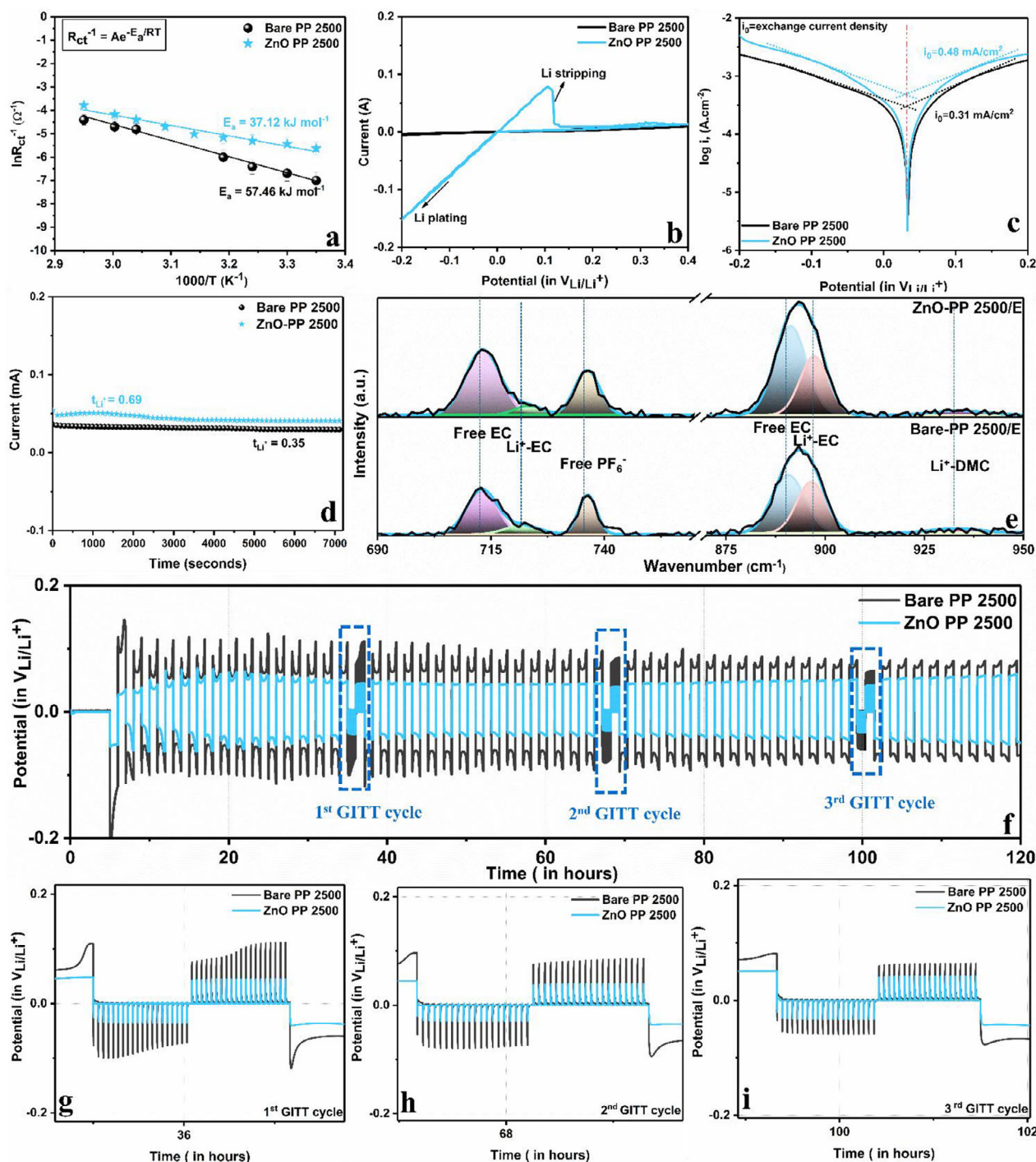
Figure 3. a) Activation energy test (25–65 °C), b) Cyclic voltammetry using Li|Li symmetric cell, c) Tafel plots, d) Li-ion transference number for bare and ZnO-PP. e) Raman Spectra of bare, and ZnO-PP soaked in a 1 M LiPF 6 in 1:1:1 EC:EMC: DMC. f) GITT voltage-time profiles of Bare PP and ZnO-PP, zoomed image of g) GITT 1 st cycle h) GITT 2 nd cycle i) GITT 3 rd cycle.
