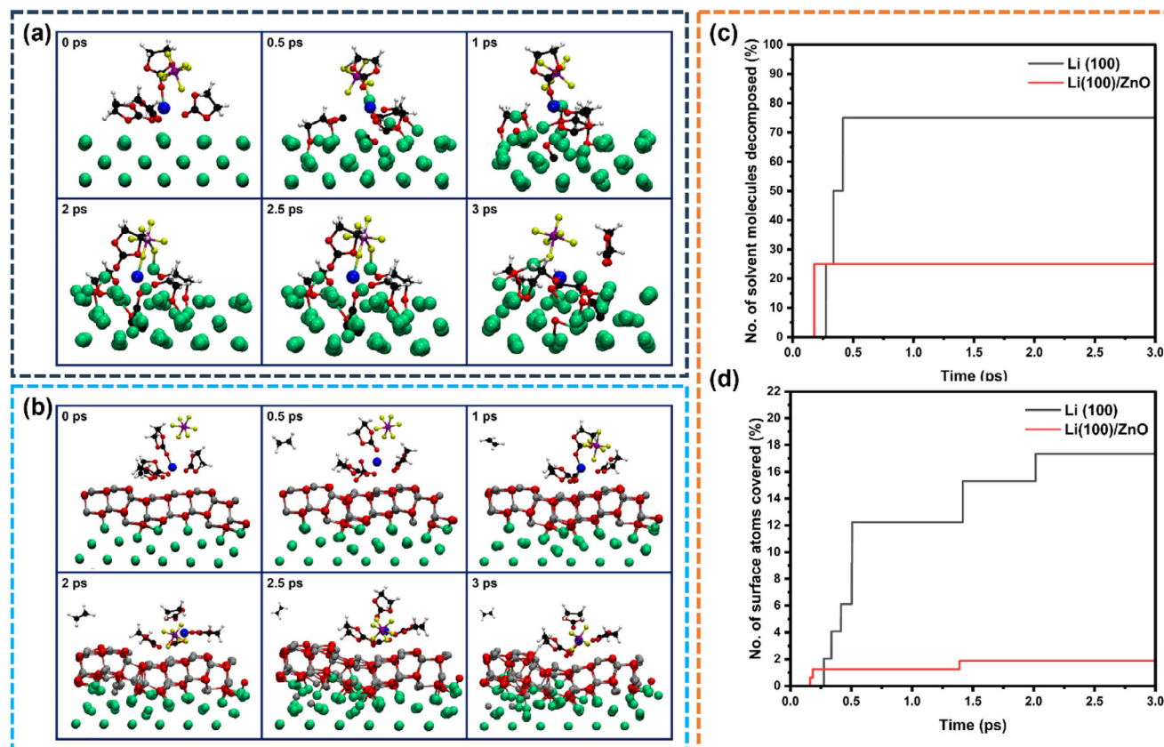
Figure 7. Snapshots from the AIMD trajectories for the electrolyte decomposition on a) Li (100) and b) Li(100)/ZnO, c) percentage of solvent molecules decomposed on the surface as a function of time, here, a solvent molecule is considered to be decomposed only when the C–O bond distance of the solvent is greater than 1.9 Å and Li/Zn (surface)-C/O distance is less than 2.4 Å, and d) percentage of surface atoms on which the decomposition products are adsorbed as a function of time. The atoms in the first two layers of Li (100) and Li(100)/ZnO are considered as surface atoms for this analysis. Here, a surface Li atom is considered to be covered by the decomposition product if the Li/Zn(surface)-C/O (EC) distance is less than 2.4 Å. Atom color codes: yellow (F), green (surface Li), blue (adsorbed Li), red (O), white (H), black (C), purple (P), grey (Zn).
