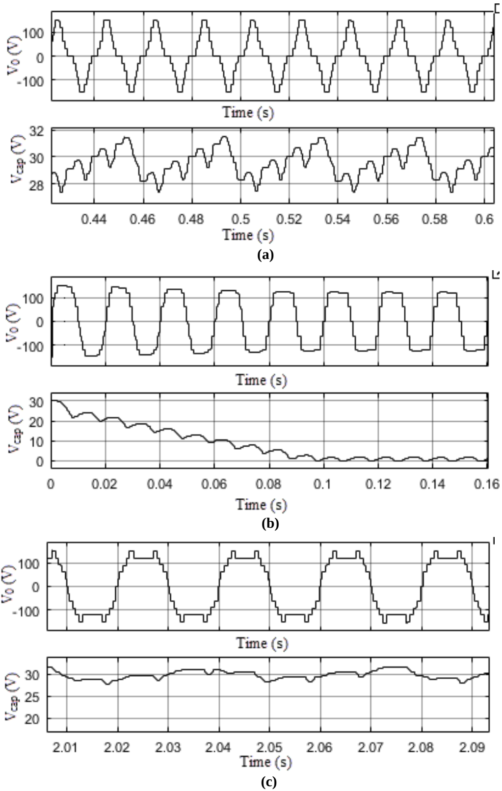
Fig. 4.10 Simulation results of MGWO optimized HC-MLI (Capacitor voltages). (a) V_0 and V_{cap} for modulation index ( m_a ) = 0.6. (b) V_0 and V_{cap} for m_a = 1.1 in case of unbalanced condition of capacitor. (c) V_0 and V_{cap} for m_a = 1.1 at balanced condition of capacitor voltage.
