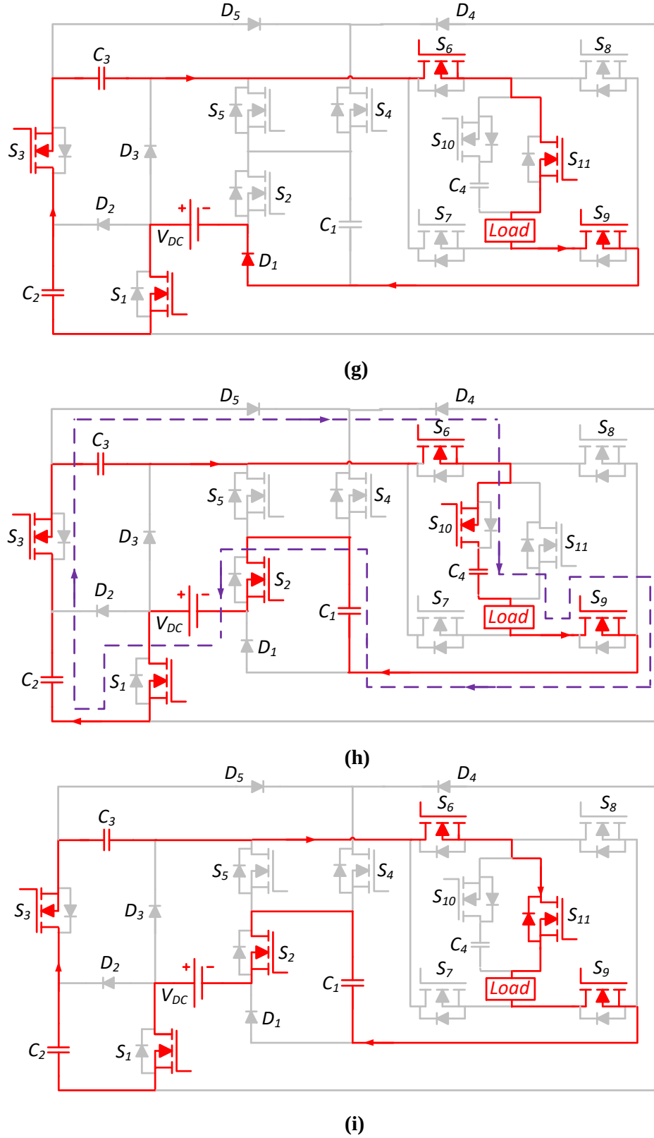
Fig. 5.3 Current flow for positive voltage levels of the proposed 17-level DASC-MLI. (a) Current flow at voltage level zero. (b) Current flow at voltage level V_{DC}/2 . (c) Current flow at voltage level V_{DC} . (d) Current flow at voltage level 3V_{DC}/2 . (e) Current flow at voltage level 2V_{DC} . (f) Current flow at voltage level 5V_{DC}/2 . (g) Current flow at voltage level 3V_{DC} . (h) Current flow at voltage level V_{DC}/2 . (i) Current flow at voltage level 4V_{DC} .
