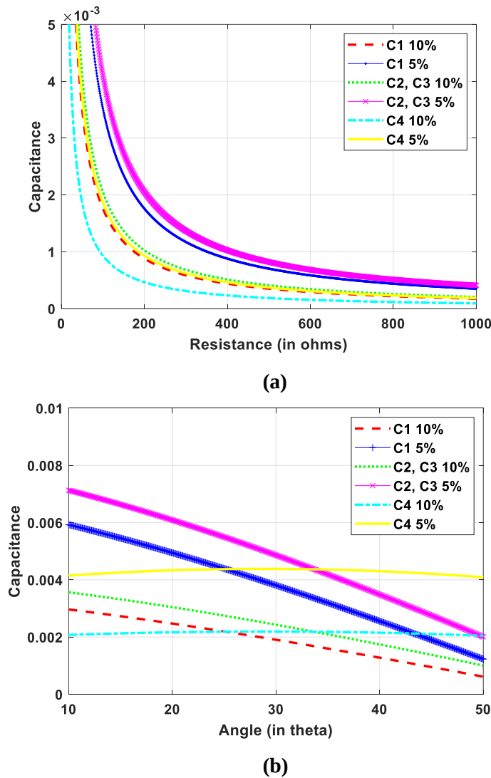
Fig. 5.6 Values of capacitance of all capacitors. (a) under different load resistance. (b) under different phase angles.
