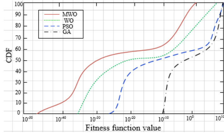
Fig. 3.5 Rate of convergence comparison of WO, PSO and GA algorithms.
