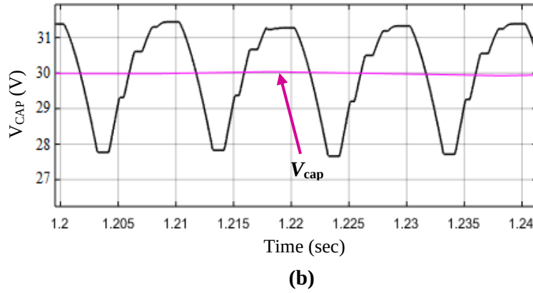
Fig. 2.15 Simulation results of three-phase capacitor voltages. (a) Three-phase capacitor voltages with voltage averaging. (b) Capacitor voltage with voltage averaging ( V_{CAP} ).
