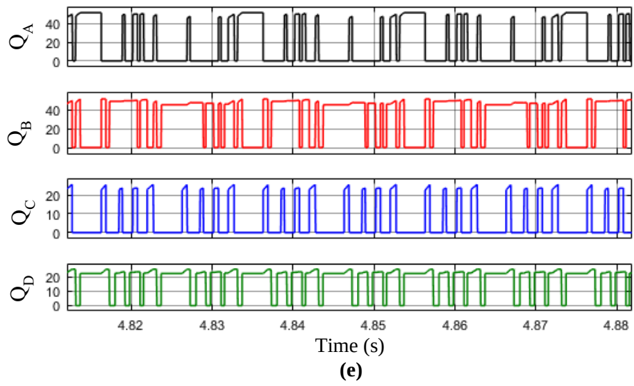
Fig. 6.8 Simulation results of voltage stress of the proposed RVSC-MLI. (a) Voltage stresses across switches ( S_1, S_2 and S_3 ). (b) Voltage stresses across switches ( S_4 and S_5 ). (c) Voltage stresses across switches ( S_a, S_b, S_c and S_d ). (d) Voltage stresses across switches ( T_1, T_2, T_3 and T_4 ). (e) Voltage stresses across switches ( Q_A, Q_B, Q_C and Q_D ).
