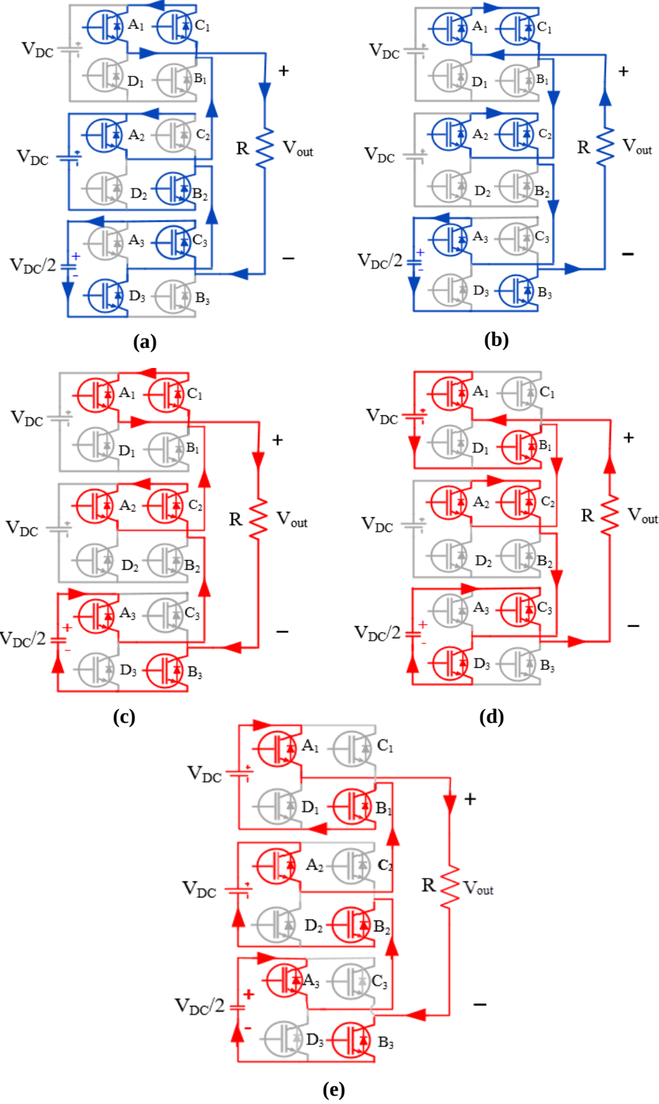
Fig. 2.7 Capacitor voltage balancing conditions. Charging interval I_{load} > 0 . (b) Charging interval I_{load} < 0 . (c) Discharging interval I_{load} > 0 . (d) Discharging interval I_{load} < 0 . (e) Discharging interval ( t_3 ) of peak voltage.
