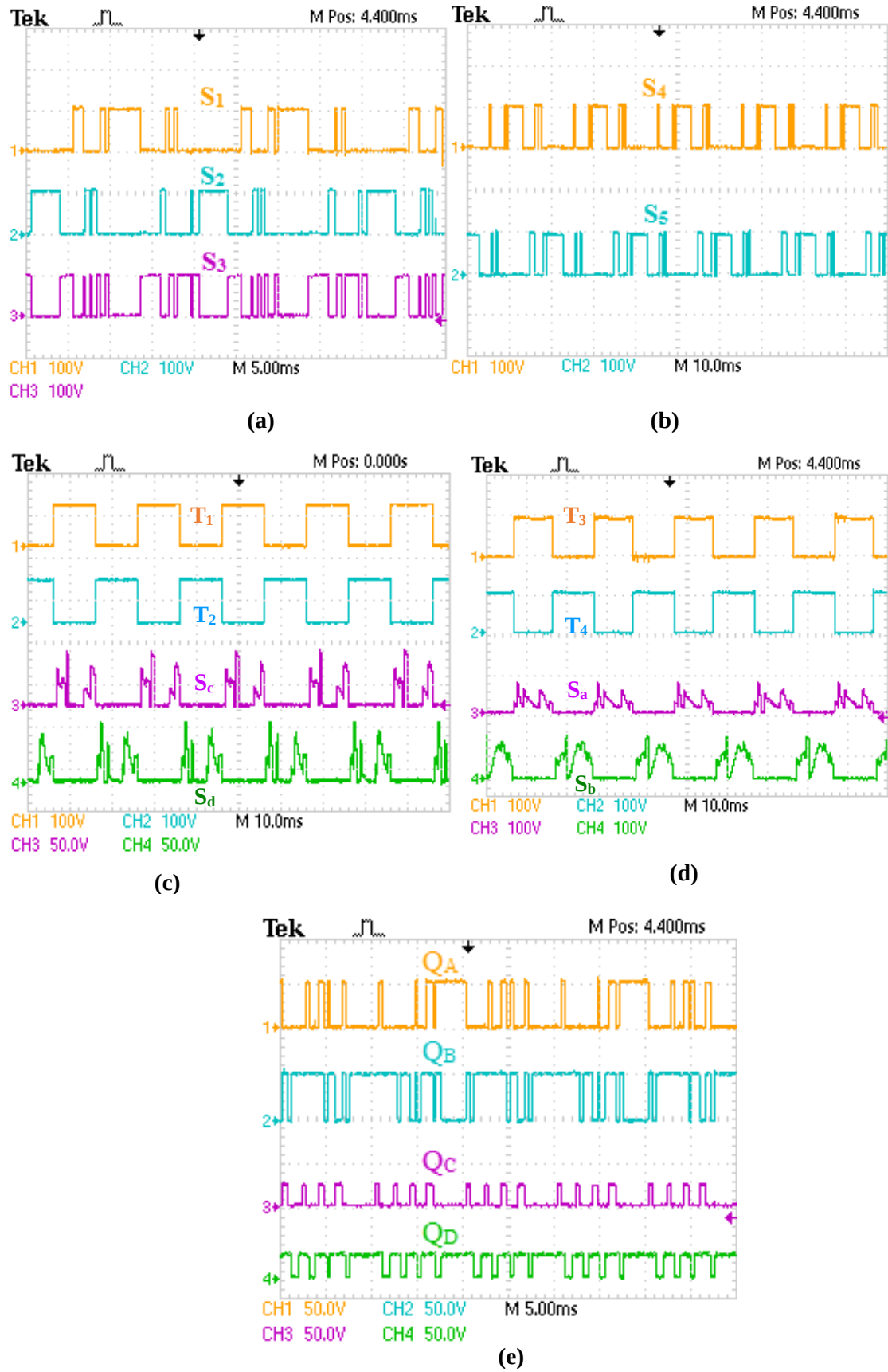
Fig. 6.12 Experimental results of voltage stresses of the proposed RVSC-MLI. (a) Voltage stresses across switches ( S_1 , S_2 , S_3 ). (b) Voltage stresses across switches ( S_4 , S_5 ). (c) Voltage stresses across switches ( T_1 , T_2 , S_c , S_d ). (d) Voltage stresses across switches ( T_3 , T_4 , S_a , S_b ). (e) Voltage stresses across switches ( Q_A , Q_B , Q_c , Q_D ).
