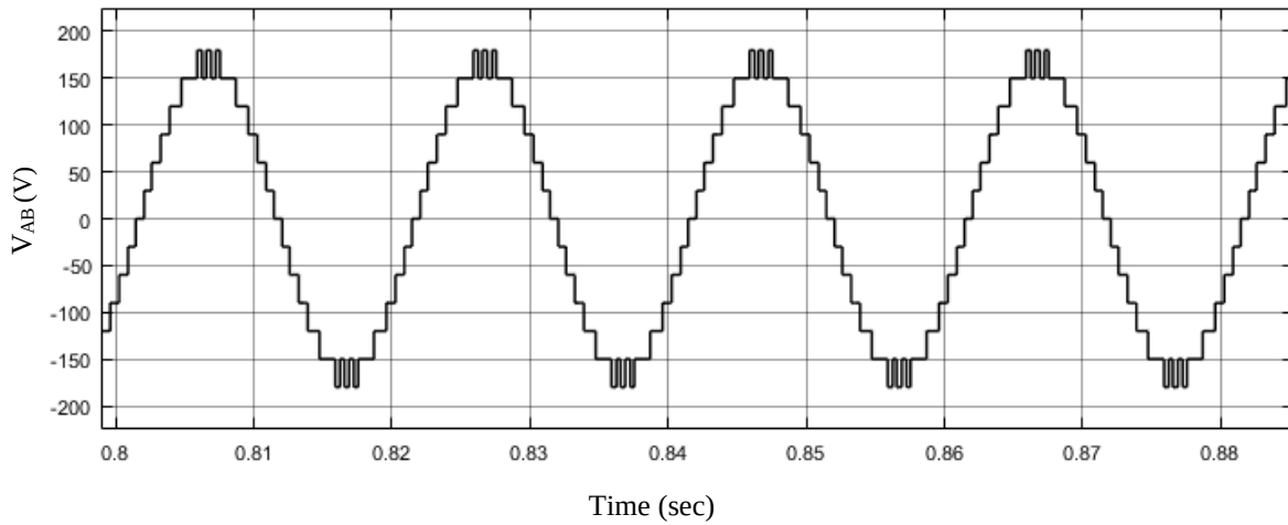
Fig. 2.17 Output voltage ( V_{AB} ) at m_a = 0.55 .
