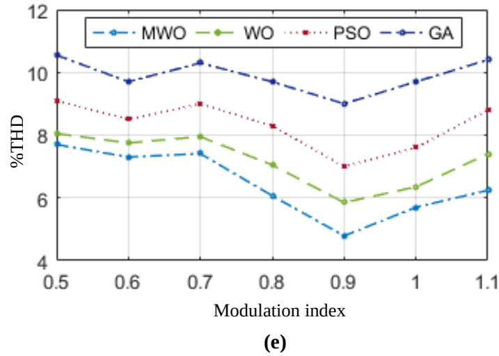
Fig. 3.6 Comparison between harmonics of different algorithms (GA, PSO, WO and MWO). (a) Magnitude of 5 th harmonic. (b) Magnitude of 7 th harmonic. (c) Magnitude of 11 th harmonic. (d) Magnitude of 13 th harmonic. (e) %THD of GA, PSO, WO and MWO.
