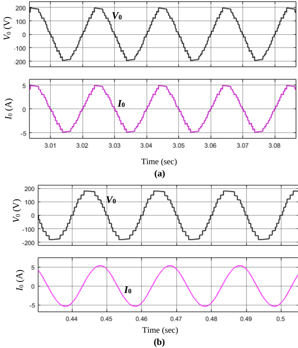
Fig. 6.6 Simulation results of the proposed 17-level RVSC-MLI. (a) Output voltage ( V_o ) and current ( I_o ) for R load ( R = 40 \Omega ). (b) Output voltage ( V_o ) and current ( I_o ) for R - L load ( R = 40 \Omega , L = 60 \text{ mH} ).
