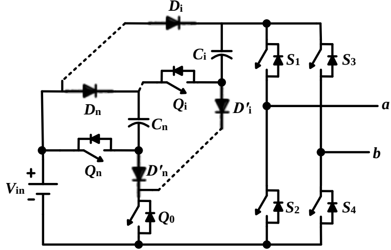
Fig. 1.9 Topology of the proposed switched capacitor MLI [40].
