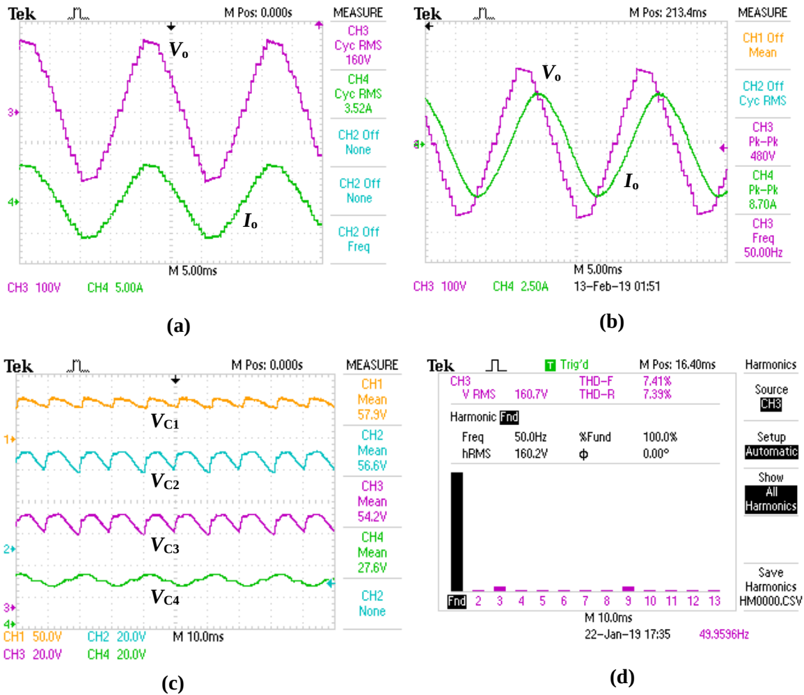
Fig. 5.13 Experimental results of the proposed DASC-MLI. (a) Output voltage ( V_o ) and current ( I_o ) for R load ( R=40\ \Omega ). (b) Output voltage ( V_o ) and current ( I_o ) for R - L load ( R=40\ \Omega , L=100\text{ mH} ). (c) Capacitor voltages ( V_{C1} , V_{C2} , V_{C3} , V_{C4} ). (d) Harmonic spectrum of V_o .
