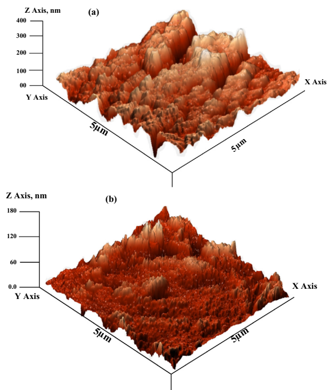
Figure 9 AFM micrographs for mild steel surface (a) in the absence and (b) in the presence of optimum concentration of Telmisartan.
