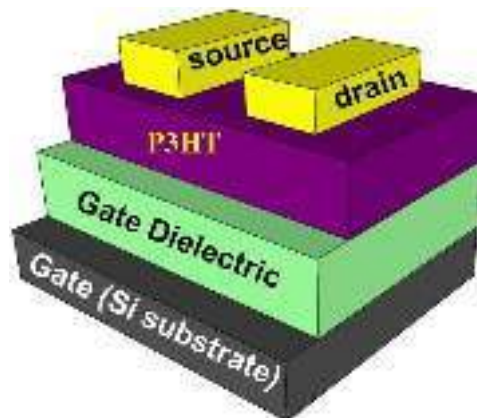
Fig. 3.1 Schematic 3-D structure of bottom-gate top-contact OFET
