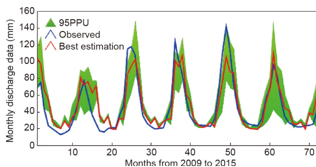
Fig. 9. Plot of estimated and observed values after calibration using SUFI-2.
