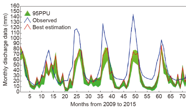
Fig. 8. Plot of estimated and observed values after calibration using GLUE.
