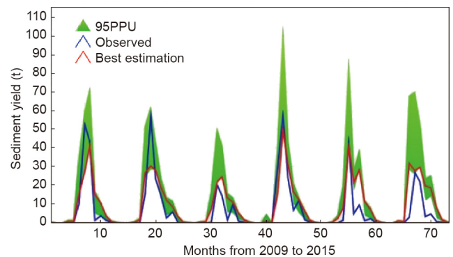
Fig. 10. Plot of estimated and observed values of sediment yield (mm).
