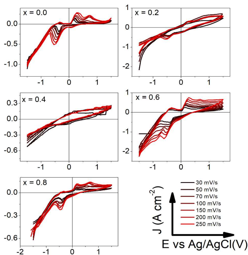
Figure 4.10: Cyclic Voltammetric curves for the (1+x) PrCoO_3 - (1-x) BaCoO_3 with the different scan rates
