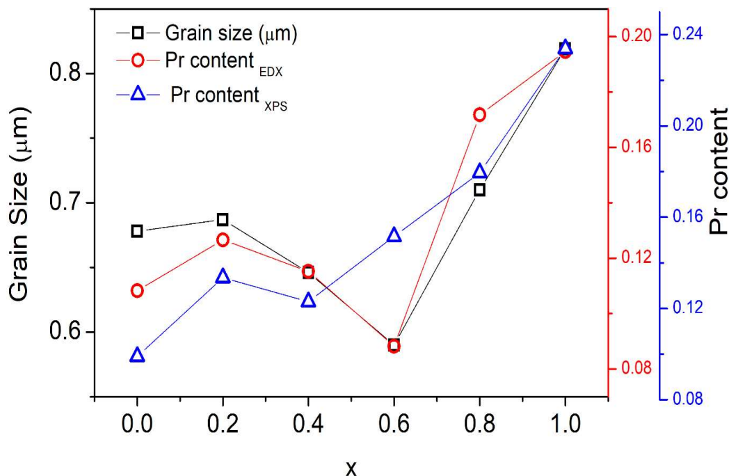
Figure 4.8: Variation of grain size obtained from Grain size histograms and Pr content observed from EDX and XPS with x
