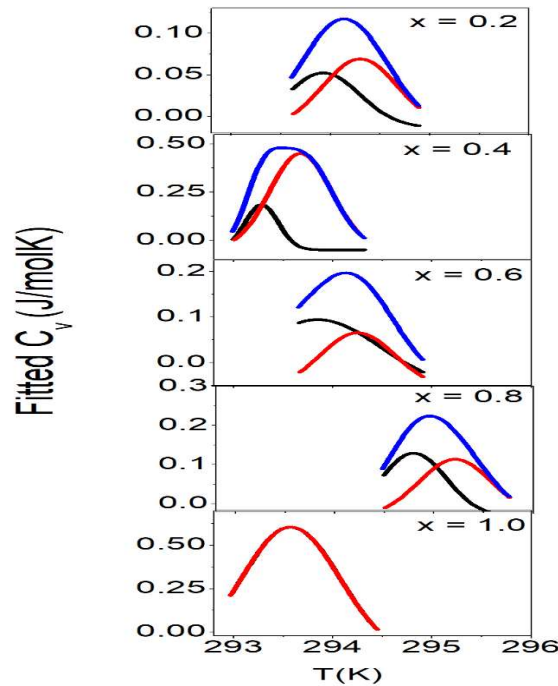
Figure 4.4: Specific heat ( C_v ) of the studied compositions (1+x) \text{PrCoO}_3 - (1-x) \text{BaCoO}_3 showing the presence of two phases \text{PrBaCo}_2\text{O}_{6-\delta} and \text{PrCoO}_3
