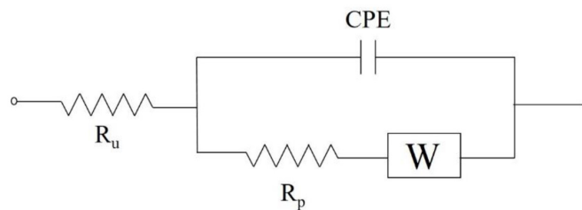
FIGURE 7.3: Equivalent electrochemical circuit of CPE model.
