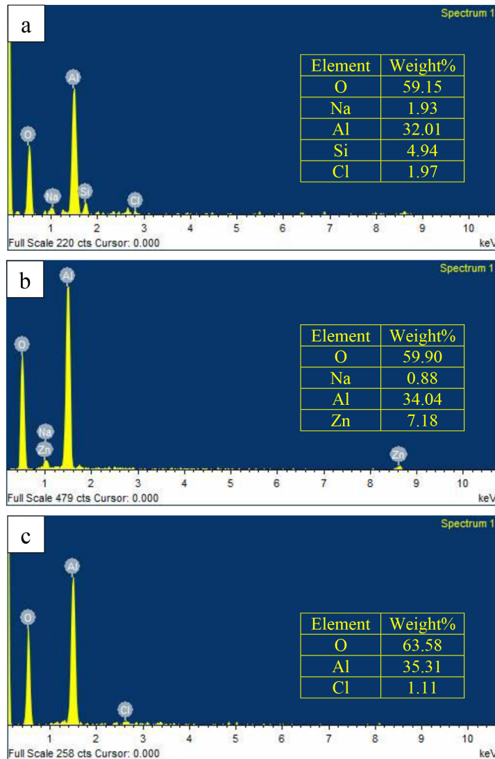
FIGURE 7.9: EDX results of the 7075 Al alloy following immersion in 3.5 wt.% NaCl solution for 15 days: (a) un-USSP, (b) USSP 15 and (c) USSP 300.
