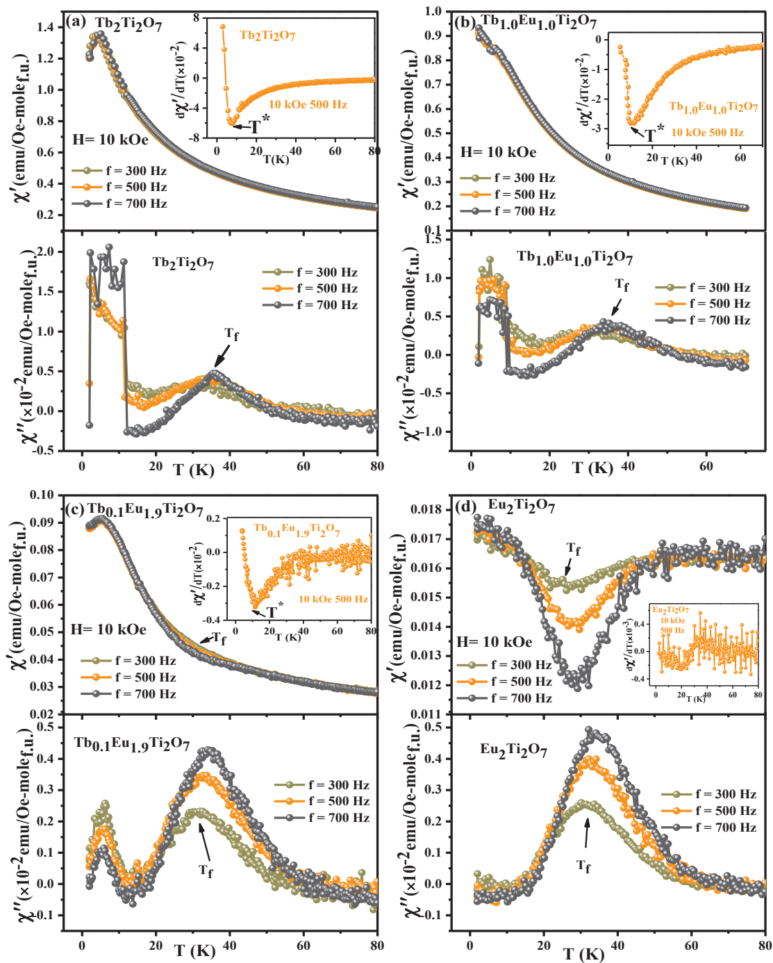
Fig. 6. \chi'(T) (upper panel) and \chi''(T) (lower panel) of TETO compounds at applied field of 10 kOe. (a) x = 0.0 , (b) x = 0.5 , (c) x = 0.95 , (d) x = 1.0 . The inset in every upper panel: d\chi'(T)/dT with T . Marked by arrow are: Single ion spin freezing peak ( T_f ) and Single moment saturation peak ( T^* ).
