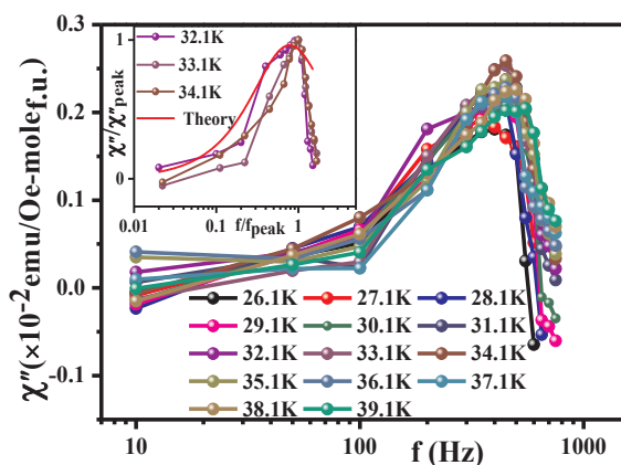
Fig. 4b. \chi''(f) at different temperatures for Tb_2Ti_2O_7 . Inset: Normalized \chi'' as a function of f/f_{peak} and fitted theoretically (red) by Casimir du pre relations at and near the transition temperature for Tb_2Ti_2O_7 . (For interpretation of the references to color in this figure legend, the reader is referred to the web version of this article.)
