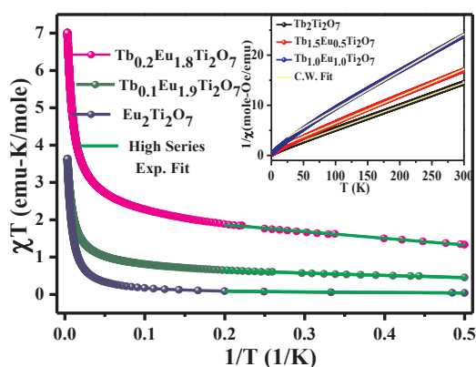
Fig. 3d. High Temperature Series Expansion fit for (Tb_{1-x}Eu_x)_2Ti_2O_7 ( x = 0.90, 0.95, 1.0 ) samples. Inset: Curie-Weiss fit for (Tb_{1-x}Eu_x)_2Ti_2O_7 ( x = 0, 0.25, 0.50 ) samples.
