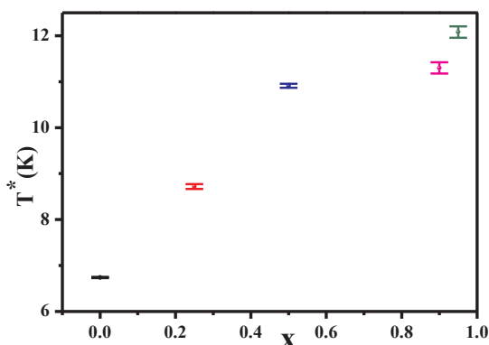
Fig. 7b. Variation of field induced transition temperature T^* with Eu content ( x ) for TETO samples.
