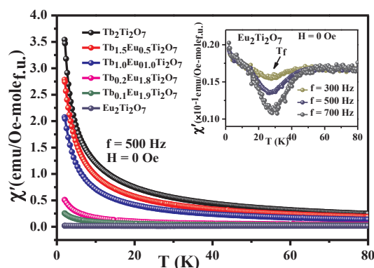
Fig. 5a. \chi'(T) of all TETO compounds measured at H = 0 Oe ( f = 500 Hz). Inset: \chi'(T) of ETO at H = 0 Oe.
