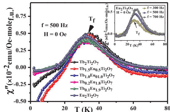
Fig. 5b. \chi''(T) of all TETO compounds measured at H = 0 Oe ( f = 500 Hz). Inset: \chi''(T) of ETO at H = 0 Oe.
