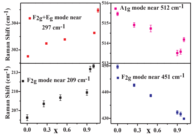
Fig. 2b. Variation of all four active phonon modes as a function of x in (Tb 1-x Eu x ) 2 Ti 2 O 7 samples.
