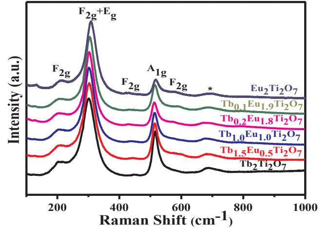
Fig. 2a. Raman Spectra of the (Tb 1-x Eu x ) 2 Ti 2 O 7 samples at 300 K.
