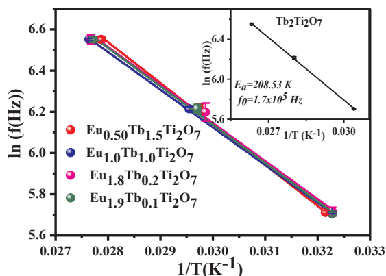
Fig. 7a. The Arrhenius Fit of ( T_f ) peak for compounds (\text{Tb}_{1-x}\text{Eu}_x)_2\text{Ti}_2\text{O}_7 ( x = 0.25, 0.50, 0.90, 0.95 ). Inset: Arrhenius Fit of \text{Tb}_2\text{Ti}_2\text{O}_7 .
