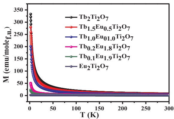
Fig. 3a. The temperature dependent magnetization (ZFC) of the (Tb_{1-x}Eu_x)_2Ti_2O_7 samples.
