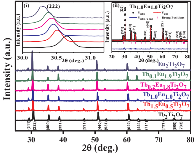
Fig. 1. Powder x-ray diffraction pattern for the (Tb 1-x Eu x ) 2 Ti 2 O 7 samples. Inset (i): Diffraction peak (222) of (Tb 1-x Eu x ) 2 Ti 2 O 7 samples. Inset (ii): Rietveld refinement for the Tb 1.0 Eu 1.0 Ti 2 O 7 sample.
