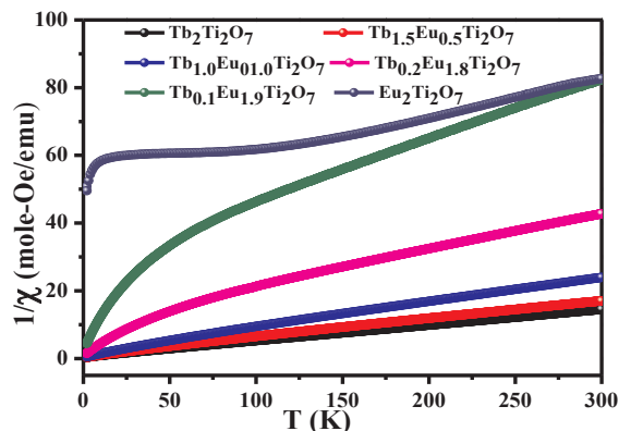
Fig. 3c. The inverse DC susceptibility of (Tb_{1-x}Eu_x)_2Ti_2O_7 samples.
