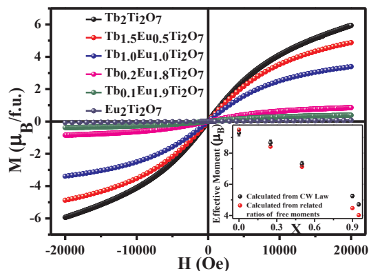
Fig. 3b. M(H) at 2 K for all TETO samples. Inset: Variation of effective magnetic moments with Eu content ( x ) derived from Curie-Weiss Law at high temperature for TETO samples.
