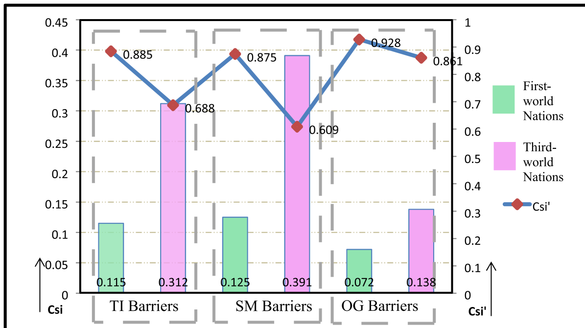
Fig. 4. Graphical representation of the coefficient of similarity.
