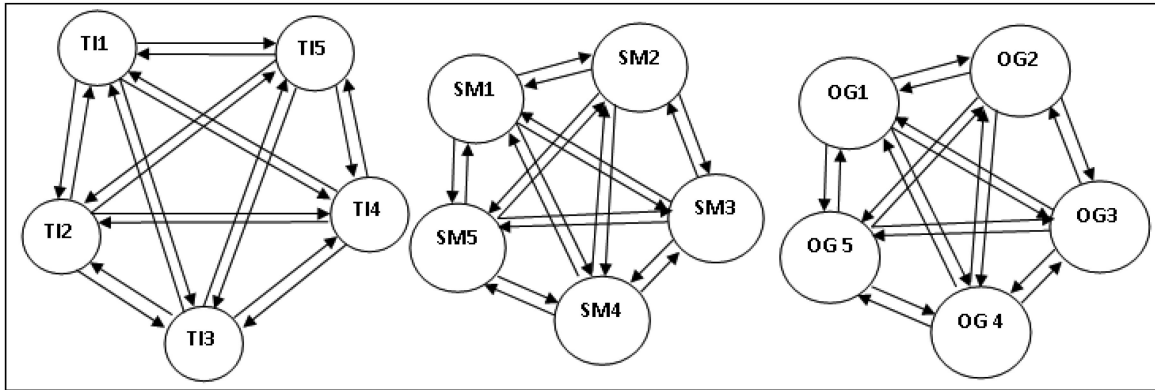
Fig. 3. Behavioral digraph of the subfactors.
