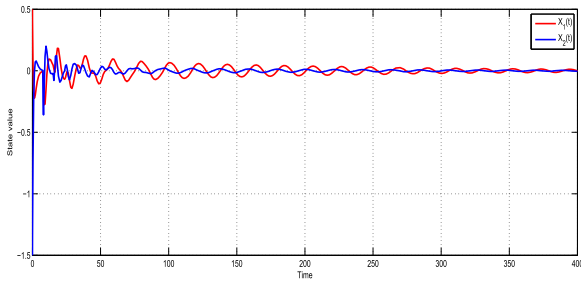
FIGURE 2. State responses of Example 2.
