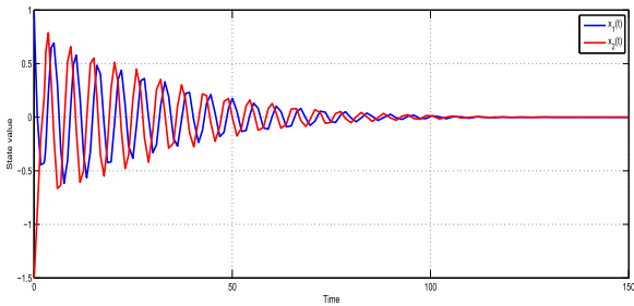
FIGURE 3. State responses of Example 3.
