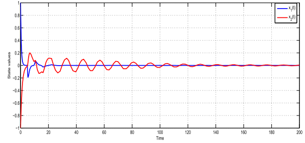
FIGURE 1. State responses of Example 1.
