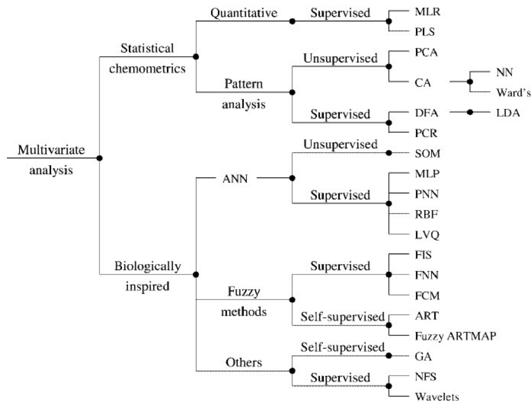
Fig.1.5 Classification scheme of the multivariate pattern analysis techniques applied to e-nose data [Pearce (2003)]
