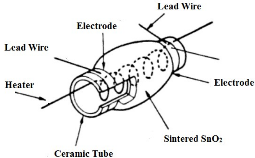
Fig. 1.4 Basic configuration of Taguchi (Figaro products) gas sensor
