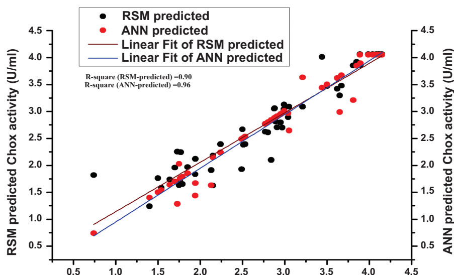
Fig. (3a). Comparison of observed and predicted ChOx concentration for RSM and ANN models.
