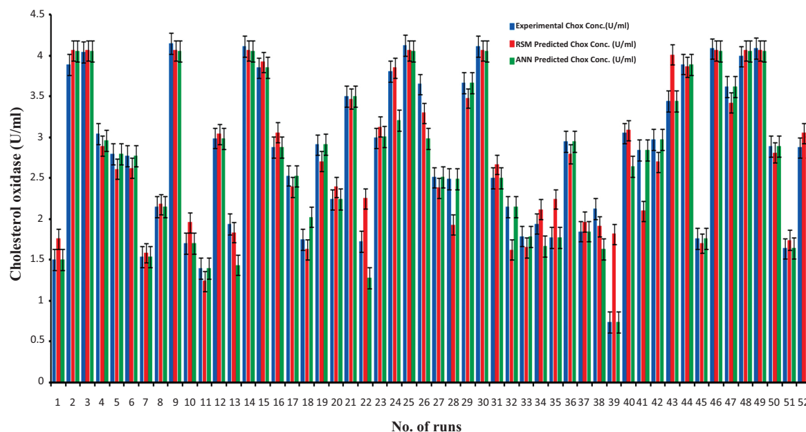
Fig. (3a). Comparison of observed and predicted ChOx concentration for RSM and ANN models.
