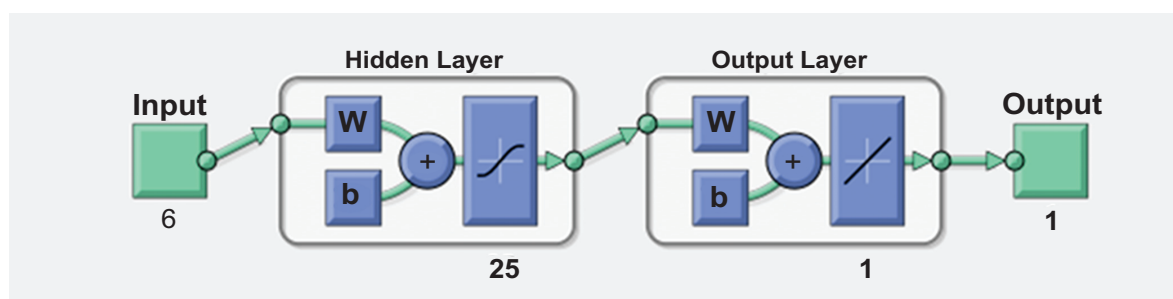
Fig. (2). Architecture of feed forward back propagation neural network. Network architecture of 6-25-1 representing the input, hidden and output layer was found to be optimum for the prediction of desired response.
