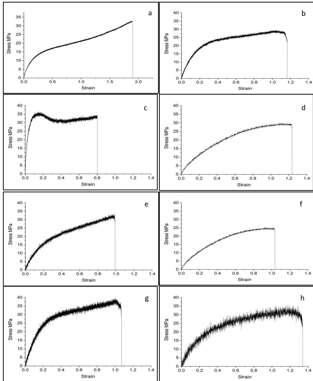
Fig. A1: Tensile stress Vs. strain curves for PVA film (a) and PVA-BPF composite films with different additives (b)-(h) ; (b)PVA-BPF film, (c) PVA-BPF film with Glutaraldehyde; (d)-(f) PVA-BPF film with Glycerol, Sorbitol and Fructose respectively; (g),(h) PVA-BPF film with Citric acid and Maleic acid respectively
