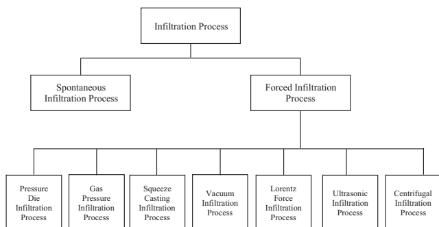
Fig. 9 – Infiltration process and its types.
