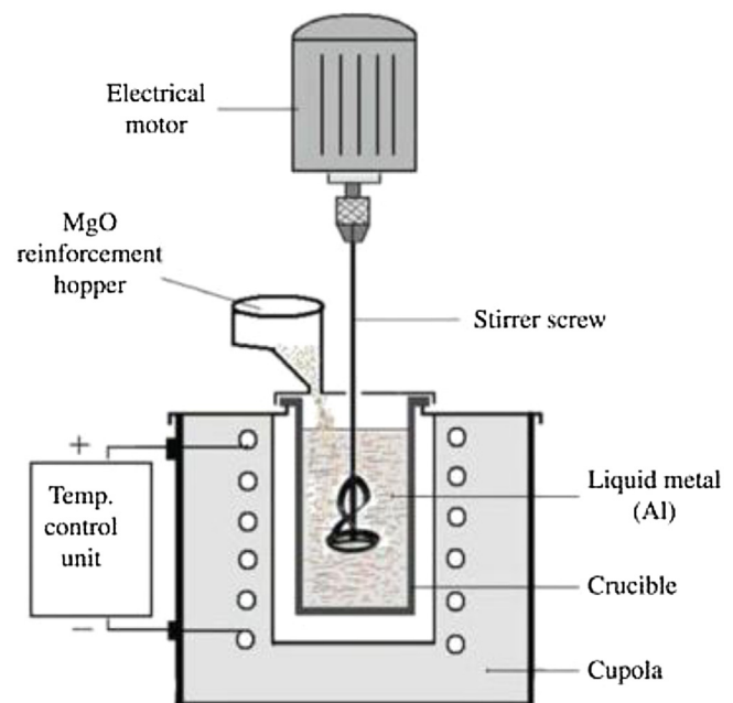
Fig. 5 – Stir Casting of MgO reinforced aluminium (Al) matrix composite.
