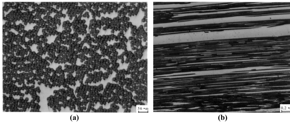
Fig. 8 – Microstructure of \text{Al}_2\text{O}_3 -Al composite processed by medium pressure infiltration at two in-plane sections [26].
