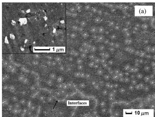
Fig. 14 – SEM analysis of particles for the in-situ \text{Al}_2\text{O}_3\text{p}/\text{Al} composites (a) distribution and morphology of particles in composites (500× and insat image at 10,000×) [43].
