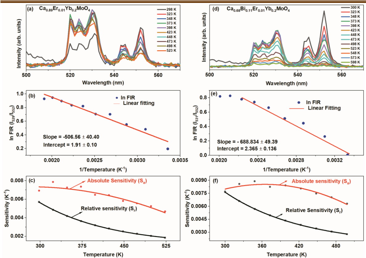
Figure 4.7 Upconversion spectra of (a) CMEY and (d) CMBEY phosphor samples at different temperatures. The logarithm of the FIR as a function of the inverse temperature for (b) CMEY, and (e) CMBEY. The relative and absolute sensitivity for (c) CMEY and (f) CMBEY samples, respectively.
