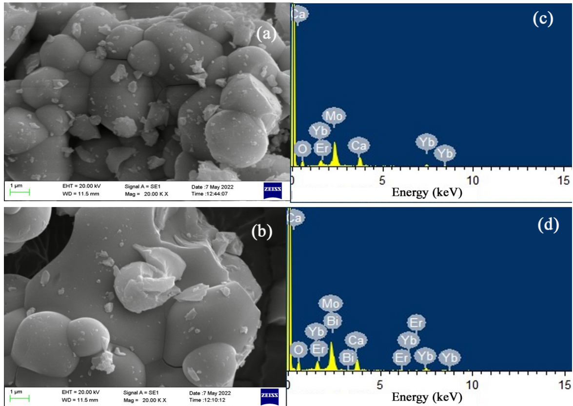
Figure 4.3 SEM image of (a) \text{Ca}_{0.79}\text{Er}_{0.01}\text{Yb}_{0.2}\text{MoO}_4 (CMEY) and (b) \text{Ca}_{0.68}\text{Bi}_{0.11}\text{Er}_{0.01}\text{Yb}_{0.2}\text{MoO}_4 (CMBEY) phosphors. The EDS spectra of (c) CMEY (d) CMBEY phosphors
