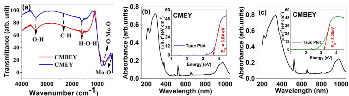
Figure 4.4 (a) Fourier transform infrared spectra of CMEY and CMBEY samples. UV-Vis-NIR absorption spectrum of (b) CMEY, and (c) CMBEY phosphors. Tauc plots of the respective UV-visible absorption spectra are provided as insets of the corresponding figures.
