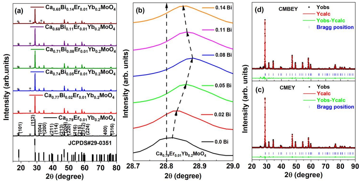
Figure 4.1 (a) XRD patterns of \text{Ca}_{0.79-x}\text{Bi}_x\text{Er}_{0.01}\text{Yb}_{0.2}\text{MoO}_4 ( x=0.00, 0.02, 0.05, 0.08, 0.11, and 0.14 ) powder samples. (b) Expanded XRD patterns of \text{Ca}_{0.79-x}\text{Bi}_x\text{Er}_{0.01}\text{Yb}_{0.2}\text{MoO}_4 ( x=0.0, 0.02, 0.05, 0.08, 0.11, and 0.14 ) powder samples between 2\theta angle 28.7 to 29.0 degree. Rietveld refined XRD patterns of (c) \text{Ca}_{0.79}\text{Er}_{0.01}\text{Yb}_{0.2}\text{MoO}_4 , and (d) \text{Ca}_{0.68}\text{Bi}_{0.11}\text{Er}_{0.01}\text{Yb}_{0.2}\text{MoO}_4 powder samples.
