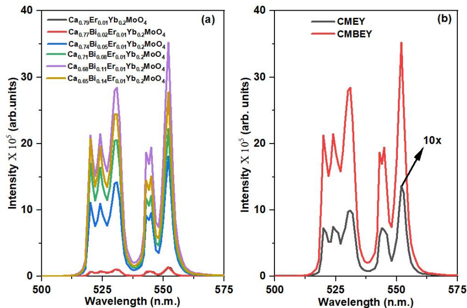
Figure 4.5 (a) UC emission of powder samples of \text{Ca}_{0.79-x}\text{Bi}_x\text{Er}_{0.01}\text{Yb}_{0.2}\text{MoO}_4 , with varying Bi concentrations ( x=0.00, 0.02, 0.05, 0.08, 0.11, \text{ and } 0.14 ), (b) comparison of the UC emission spectra of CMEY and CMBEY samples both using 980 nm laser as excitation source.
