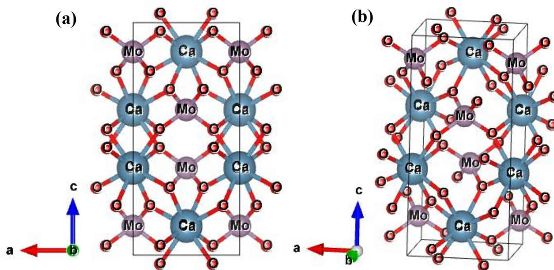
Figure 4.2 Tetragonal crystal structure of Ca 0.79 Er 0.01 Yb 0.2 MoO 4 in two different orientation obtained after Rietveld refinement of the XRD patterns.
