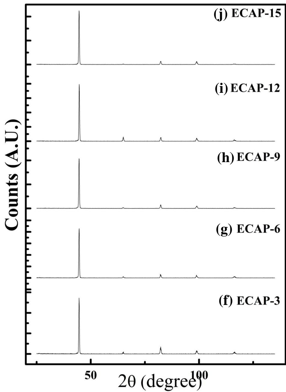
A-Figure 1: The intensity data (in arbitrary units of intensities) for the as-received and ECAPed samples against the diffraction angle 2\theta .
