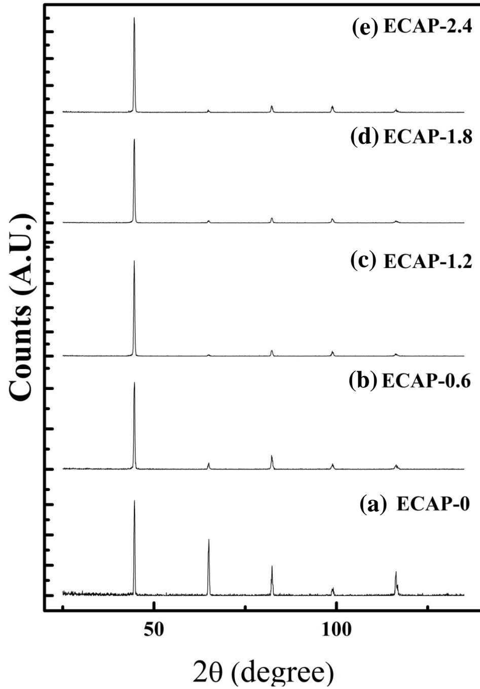
A-Figure 1: The intensity data (in arbitrary units of intensities) for the as-received and ECAPed samples against the diffraction angle 2\theta .
