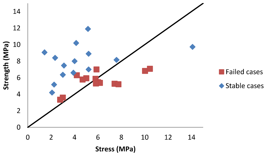
Fig. 3.6 Numerical pillars strength and stress
