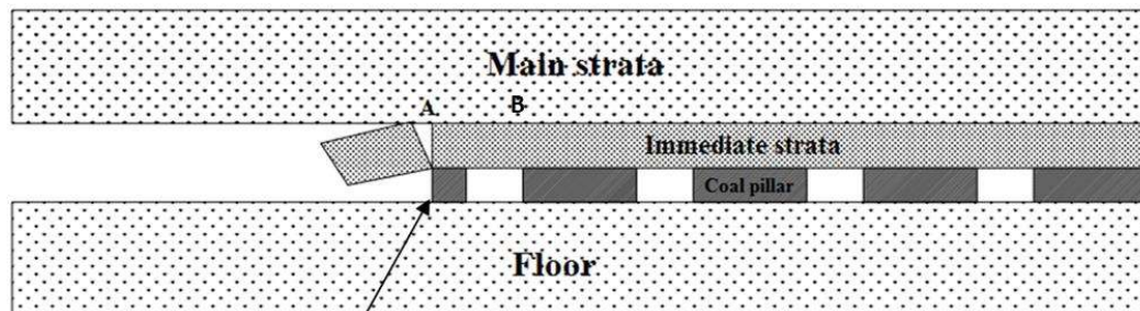
a. Maximum tensile stress at location 'A'
