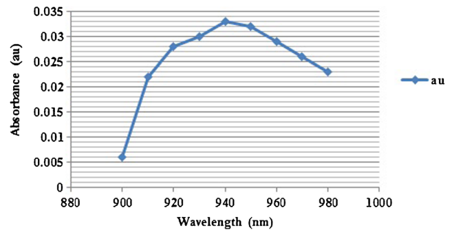
Fig. 1 Absorption spectra of glucose in distill water between 900 and 980 nm
