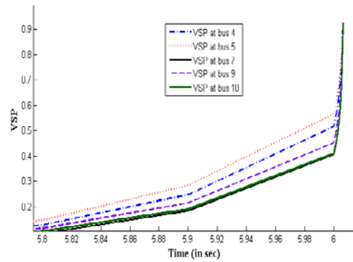
Figure 9. Closer view of VSP of Figure 8
