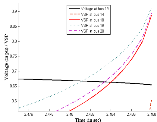
Figure 11. Closer view of Figure 10
