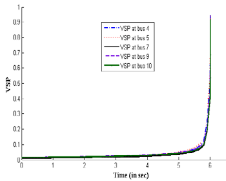
Figure 8. VSP plot for load increase at all the buses
