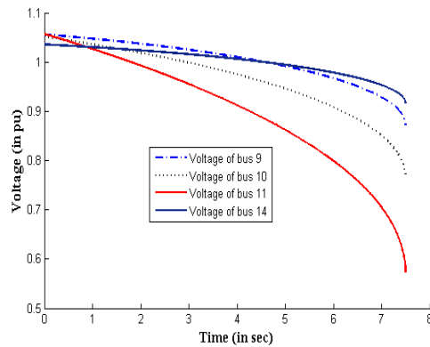
Figure 4. Critical bus voltages due to increase load at bus 11
