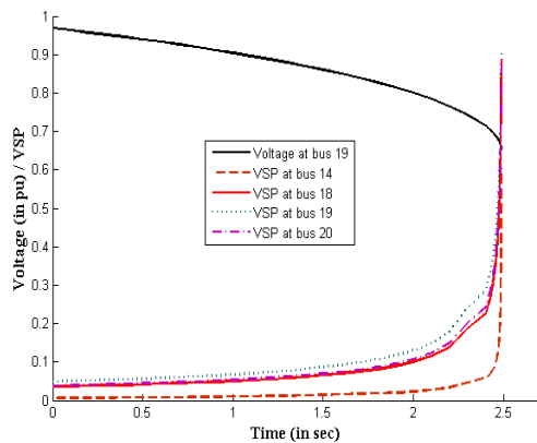
Figure 10. Change in voltage/VSP vs time at Bus 19, -14, -18 and -20 for IEEE 30-bus test system
