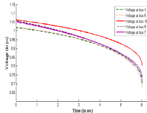
Figure 7. Critical bus voltages due to increase loads at all the load buses
