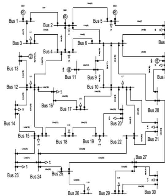
Figure 3. IEEE 30-bus test system
