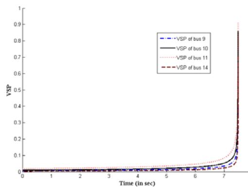
Figure 5. VSP plot for load increase at bus 11
