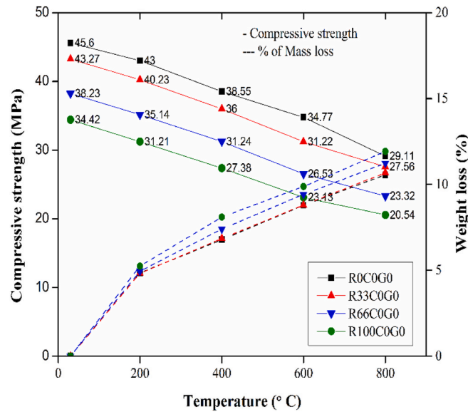
(a) Compressive strength of RAC with mass loss at varying temperature
