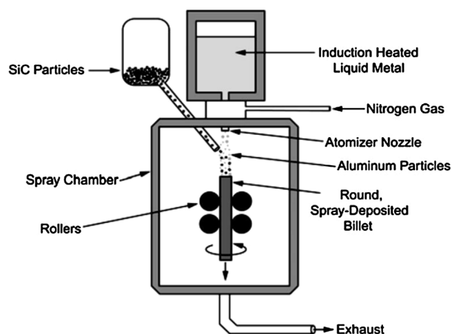
Fig. 15 – The spray deposition process [47].
