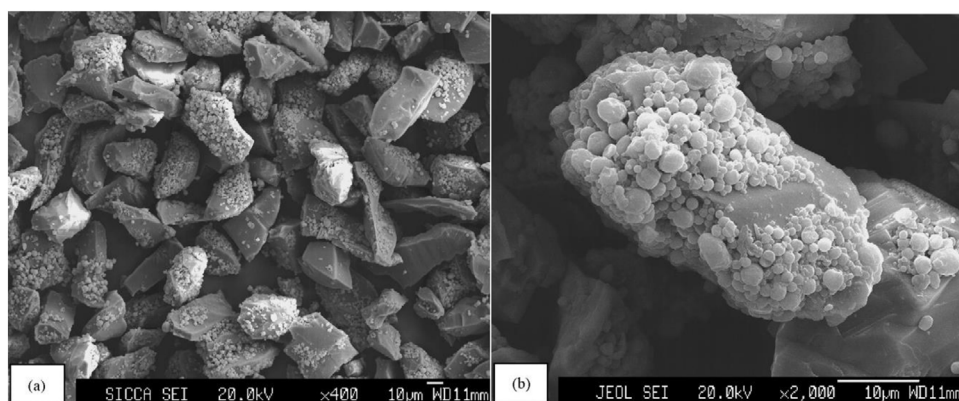
Fig. 17 – SEM micrographs of \text{Al}_2\text{O}_3 -Al composite powders fabricated by plasma spraying at 400 \times and 2000 \times [52].
