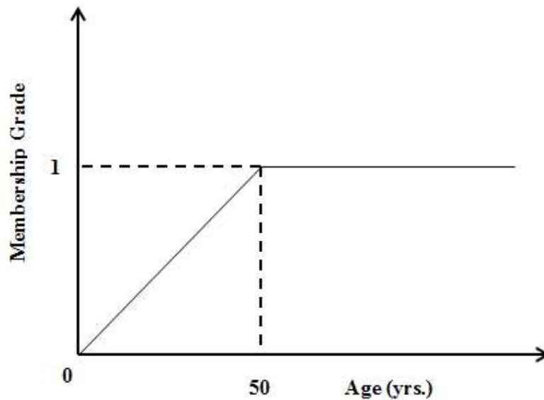
Fig. 1.1: Pictorial Representation of degree of membership
