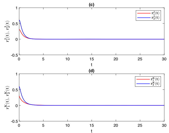
FIGURE 6 | Time response of state variables (c) r_1^I, r_2^I and (d) r_1^K, r_2^K of the system (12) with J_1^I, J_2^I, J_1^K and J_2^K = 0 . [Colour figure can be viewed at wileyonlinelibrary.com ]
