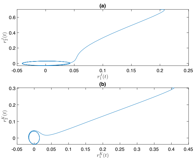
FIGURE 8 | Phase plot of state variables (a) r_1^J, r_2^J and (b) r_1^K, r_2^K of the system (13). [Colour figure can be viewed at wileyonlinelibrary.com ]
