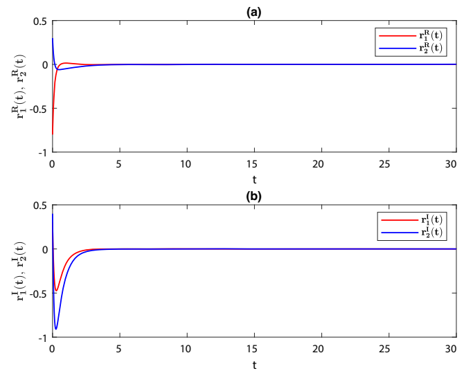
FIGURE 5 | Time response of state variables (a) r_1^R, r_2^R and (b) r_1^I, r_2^I of the system (12) with J_1^R, J_2^R, J_1^I and J_2^I = 0 . [Colour figure can be viewed at wileyonlinelibrary.com ]
