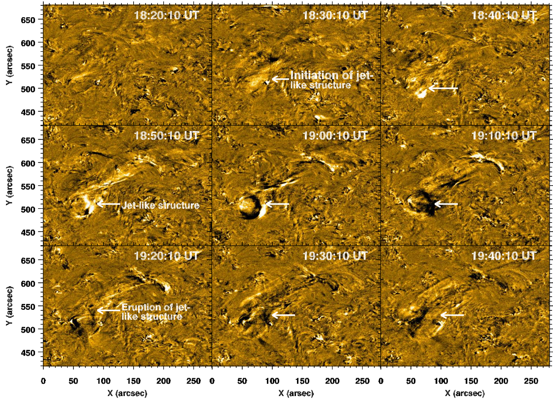
Figure 7.4: The region of interest to observe the jet-like eruption as displayed in the difference images of SDO/AIA 171 Å. The difference images show that a ring-shaped rotating jet-like eruption occurred from the northward coronal hole (CH1).
