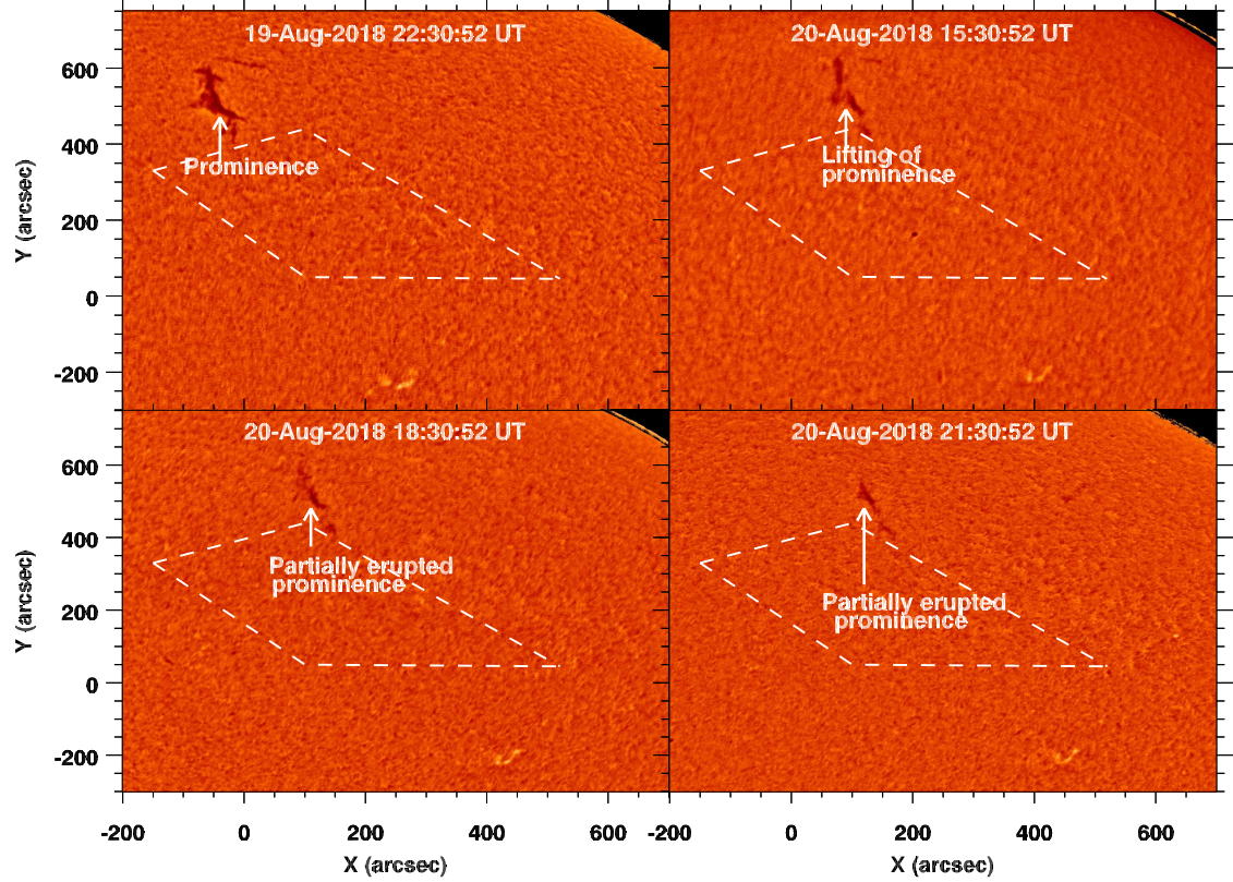
Figure 7.1: Evolution of a quiescent filament as observed by GONG/H \alpha . It evolved spatially and temporally and crossed the central meridian of the Sun on 26 August 2018. The filament was lifted and partially erupted when it passes over the northward lying coronal hole. The coronal plasma channel (CPC) is associated with the filament in its southwest direction, and its location is shown in the white box . It appears to be empty as no traces of cool plasma in H \alpha has been found in CPC, and it is only visible in the coronal emissions.
