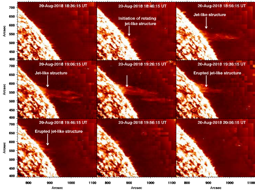
Figure 7.5: The same region of interest as Figure 7.4 in the projected plane observed by STEREO-A/EUVI-304 Å. Initiation grew and an eruption of the jet-like structure was observed in the STEREO-A/EUVI-304 Å data.
