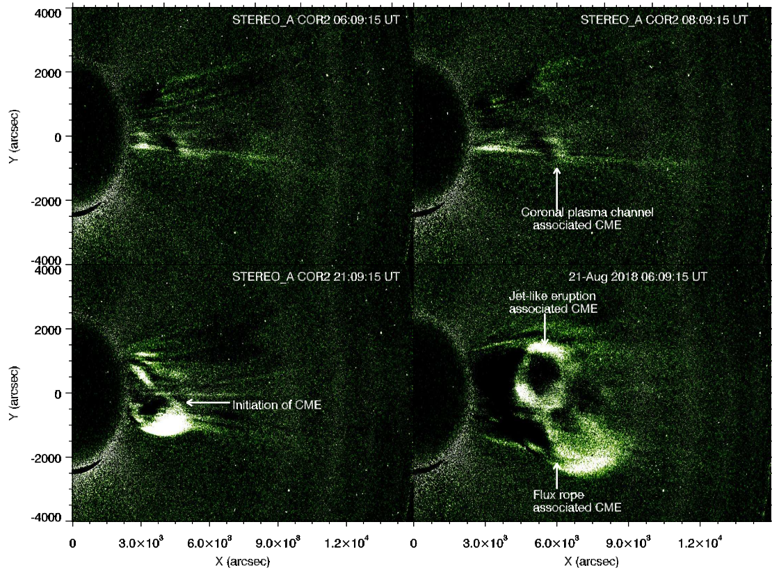
Figure 7.8: Half FOV of STEREO-A/COR2 to observe the eruption of the CMEs. A coronal-plasma channel associated CME appeared first with its low coronal signature (upper panel). The CMEs associated with the flux rope and rotating jet-like eruption have been observed using STEREO-A/COR2. Later these CMEs merge within each other and propagate towards the outer corona in the form of a compound CME.
