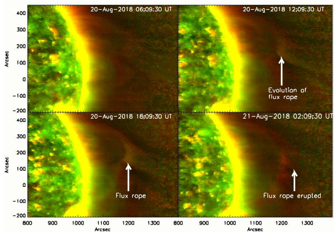
Figure 7.7: The region of interest is displayed in the STEREO-A/EUVI (171+195) Å composite images. The composite images observed the dynamics of thin and diffuse flux rope lying high in the lower corona. The top portion of the flux rope has erupted out and the lower part is connected with the solar disk ( lower panel ).
