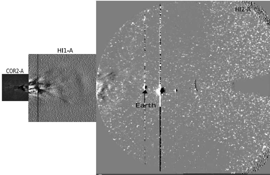
Figure 7.10: Aligned and composite images of STEREO-A/COR2 ( 2.5 - 15 R_{\odot} ), Heliospheric Imager (HI1; 15 - 90 R_{\odot} ), and Heliospheric Imager (HI2; up to 4 AU) onboard the Solar TERrestrial Relations Observatory (STEREO) on 26 August 2018 at 10:09 UT, display the interaction of CME with the Earth's magnetosphere.
