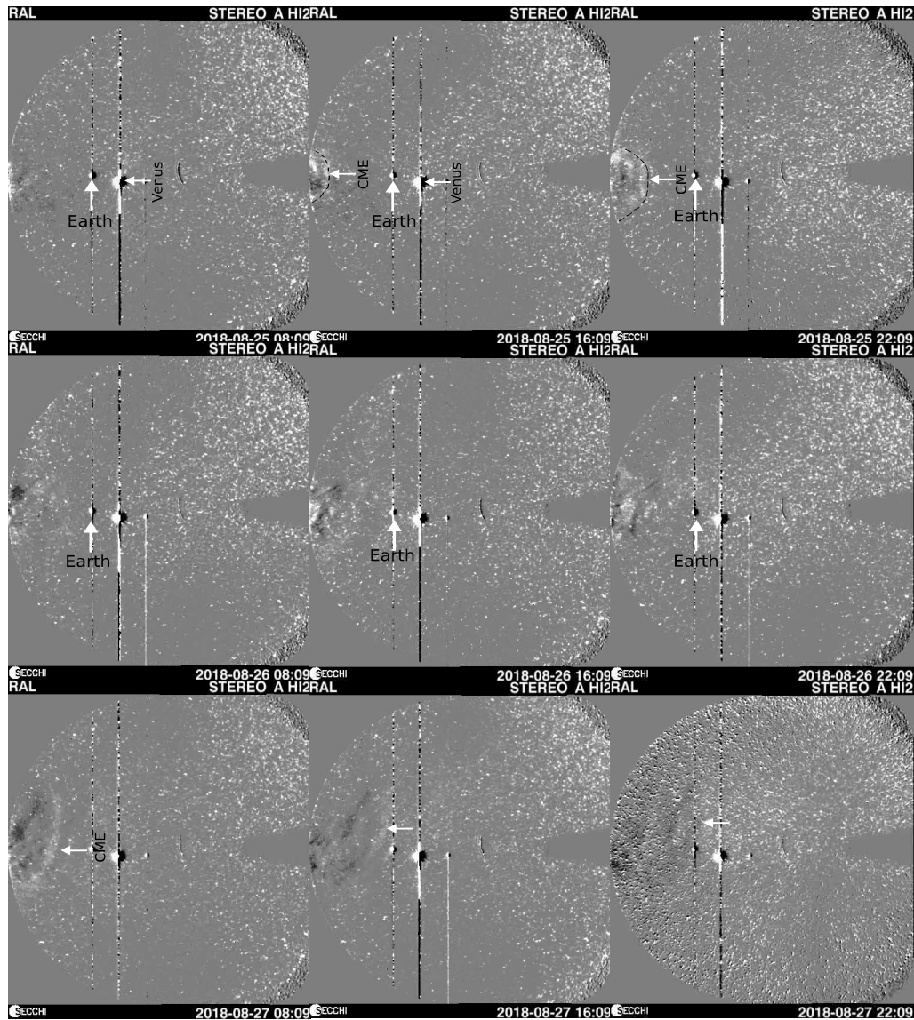
Figure 7.11: The propagation of collective CMEs towards 1 AU and interaction with the Earth's magnetosphere. The sequence of STEREO-A/HI2 images was used to observe the merged CME in interplanetary space. The observed CME moves toward 1 AU and interacts with the Earth's magnetosphere on 26 August 2018 and creates large-scale disturbances.
