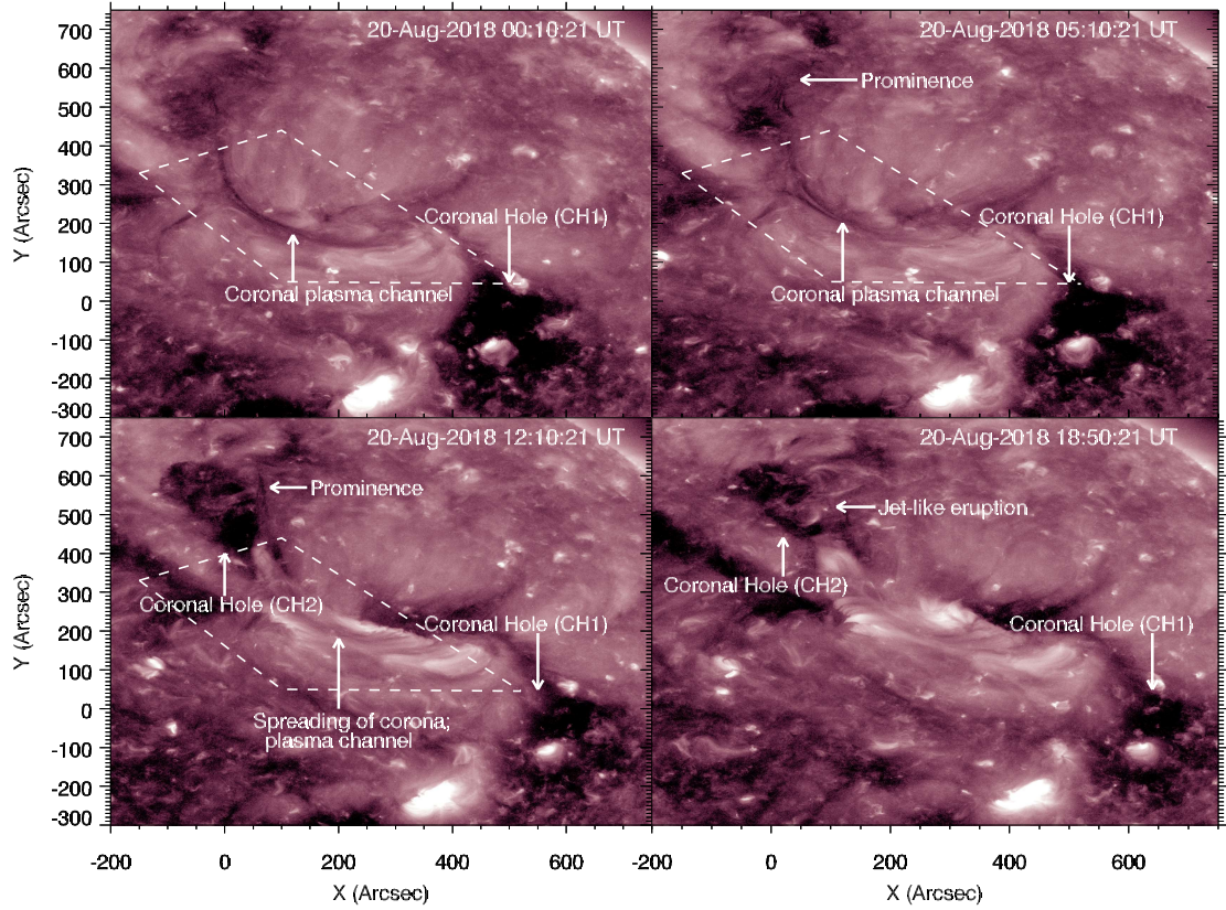
Figure 7.2: The full field of view (FOV) of the coronal plasma channel (CPC) that connects the two coronal holes (CH1 and CH2) observed by SDO/AIA 211 Å on 20 August 2018. The spreading coronal plasma channel ( white box ) and post-eruption arcade indicate that an eruption from this region has already occurred. The spreading coronal plasma channel further interacts with an open field line of a northward lying coronal hole (CH1) and may trigger a jet-like eruption ( lower panel ). The white-box-region consists of a coronal plasma channel (CPC). The impact of an eruptive coronal channel could be observed in the form of spreading of this plasma channel and formation of the post-eruption arcade as seen within the white box region .
