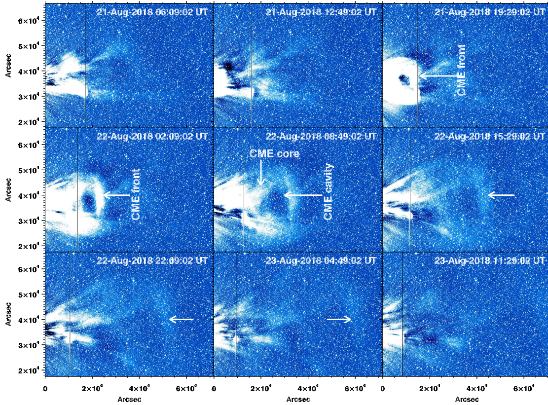
Figure 7.9: Formation of the merged CME in interplanetary space as observed by STEREO-A/HI1. The compound CME has larger angular width in interplanetary space and propagated towards the Earth. It crossed the lower interplanetary space on 23 August 2018.
