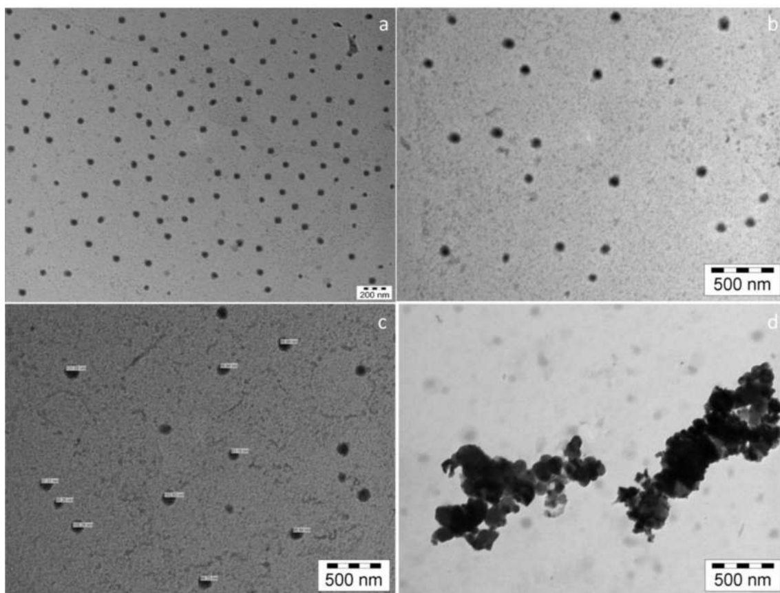
Figure 5.4. TEM images of surface-modified SCCZTOs and bare CCZTO-6h nanoparticles: (a). SCZTO-6h, (b). SCCZTO-8h (c). SCCZTO-12h and (d). CCZTO-6h nanoparticles
