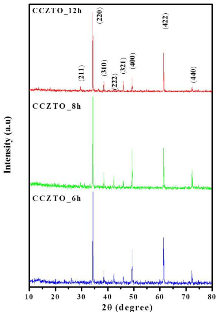
Figure 5.1. X-ray diffraction patterns of \text{CaCu}_{2.90}\text{Zn}_{0.10}\text{Ti}_4\text{O}_{12} (CCZTOs) nanoparticles
