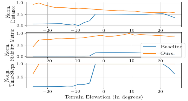
Fig. 5. Figure showing the performance metrics compared over slopes of different elevations between the baseline NN Policy and our proposed linear policy.
