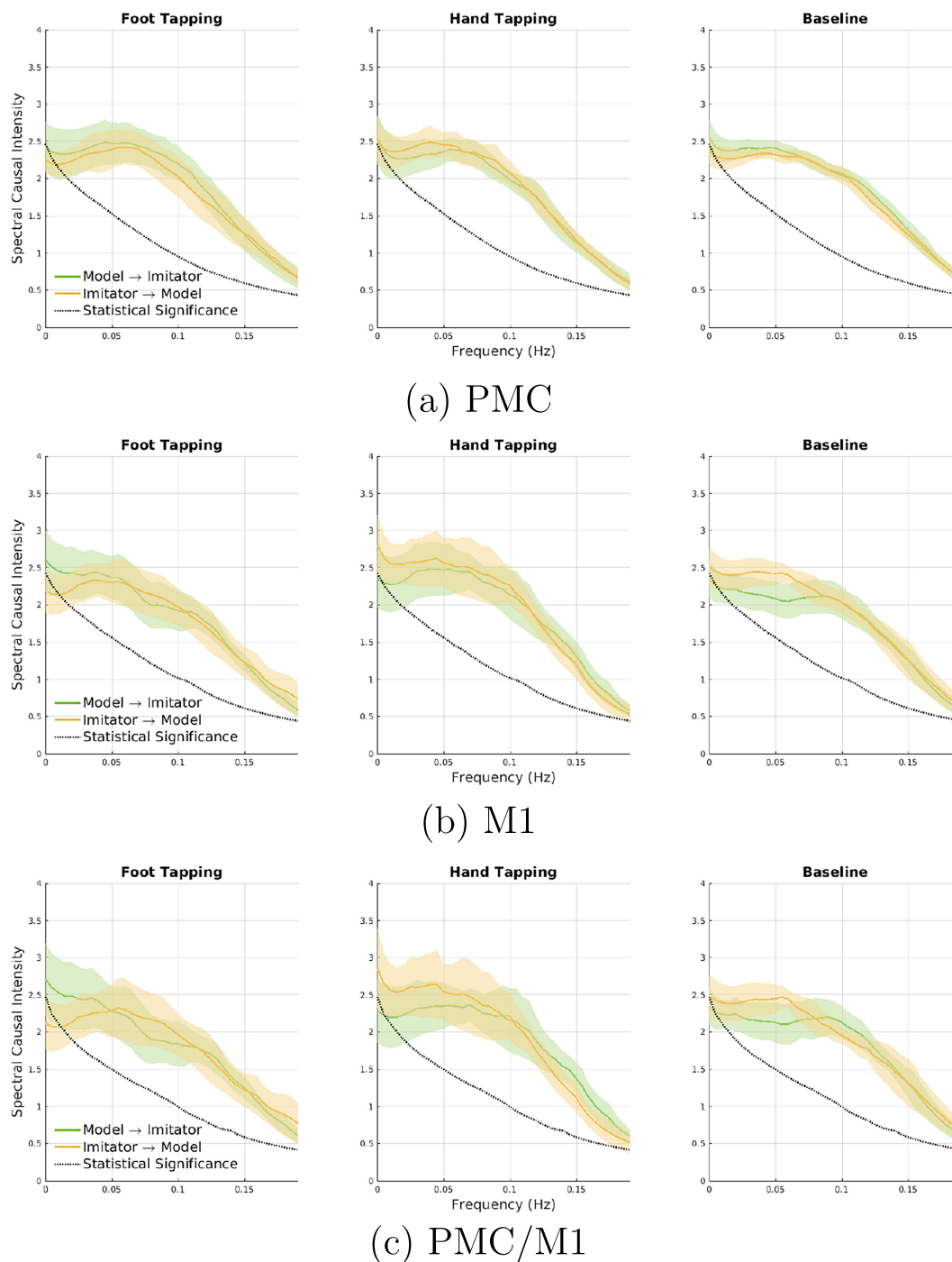
FIGURE C1 | The average and 95% confidence interval of the spectral causality of the normalized HbR time series from Model to Imitator (green plots) and from Imitator to Model (orange plots). The average is calculated for each type of event of all dyads for regions: (a) Premotor cortex (PMC), (b) Primary motor cortex (M1), and (c) PMC/M1. The statistical significance is shown in the dotted black line, which is the average spectral causality of the frequency domain surrogate data. Only spectral causality values higher than this line are considered statistically significant.
