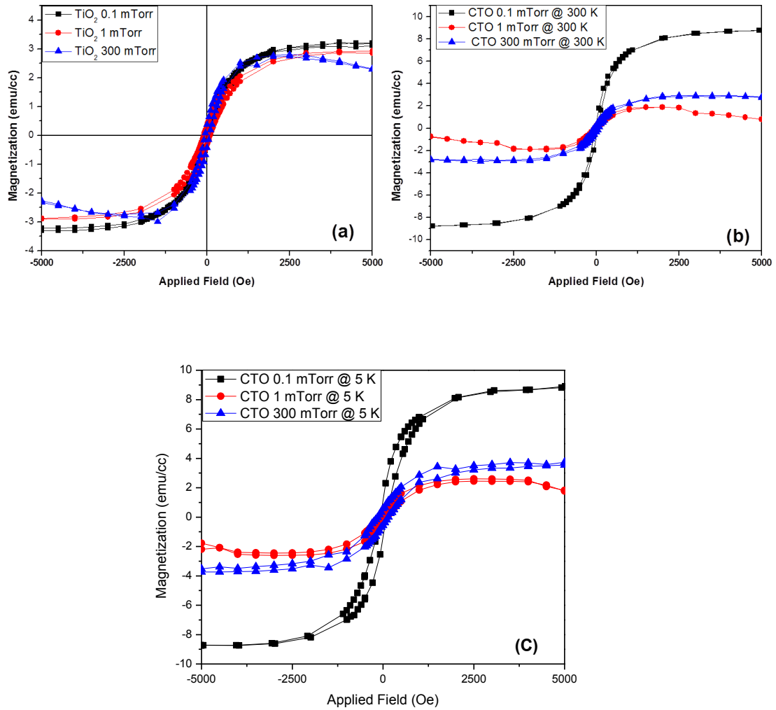
Fig.5.14 Magnetisation (M) vs. applied magnetic field (H) of: (a) TiO 2 film deposited at 0.1 mTorr, 1mTorr and 300 mTorr (at 300 K) (b) CTO films deposited at 0.1 mTorr, 1 mTorr and 300 mTorr oxygen partial pressure (at 300 K) and (C) CTO films deposited at 0.1 mTorr, 1 mTorr and 300 mTorr oxygen partial pressure (at 5 K).
