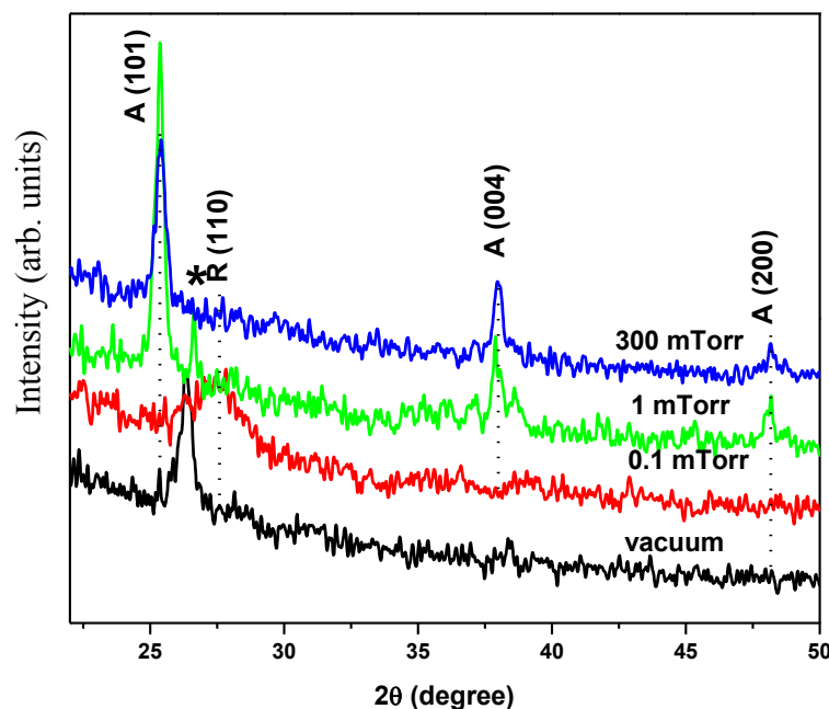
Fig.5.1. GAXRD pattern of \text{TiO}_2 thin films deposited at various oxygen partial pressures. * denotes the \text{Ti}_4\text{O}_7 phase.
