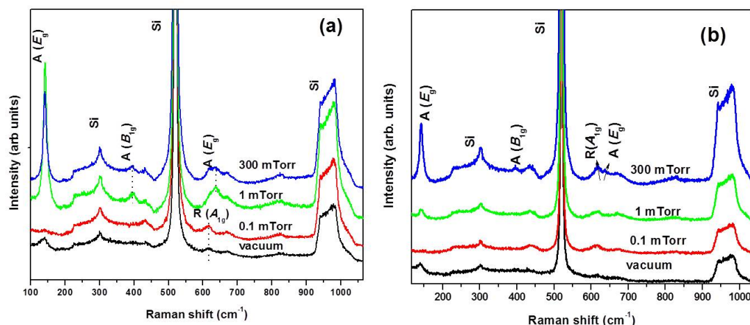
Fig.5.3 Raman spectra of (a) \text{TiO}_2 and (b) CTO films deposited at various oxygen partial pressures.
