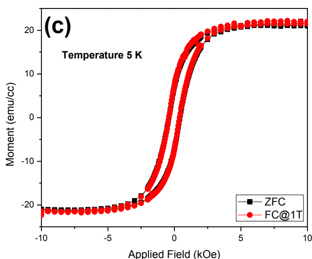
Fig.5.16 Magnetisation (M) vs. applied magnetic field (H) at 300 K of (a) CTO (b) \text{TiO}_2 films deposited at 0.1 mTorr, 1mTorr and 300 mTorr. (c) A typical M vs. H plot for CTO film deposited at 0.1 mTorr oxygen partial pressure under ZFC and FC condition.
