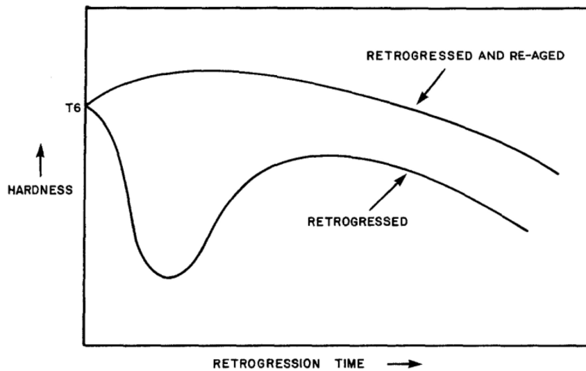
FIGURE 1.5: Variation of hardness during RRA heat treatment [12].
