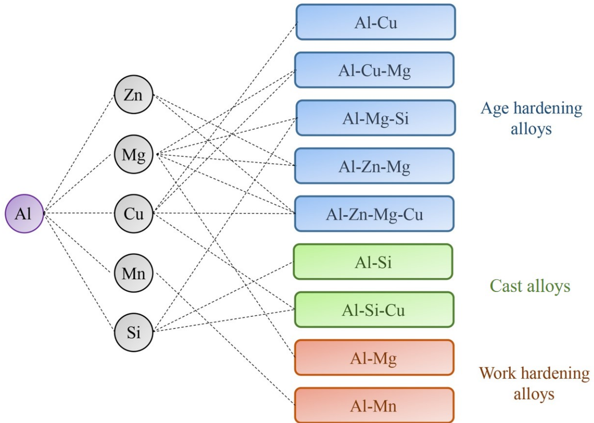
FIGURE 1.3: Primary types of aluminium alloys [8].
