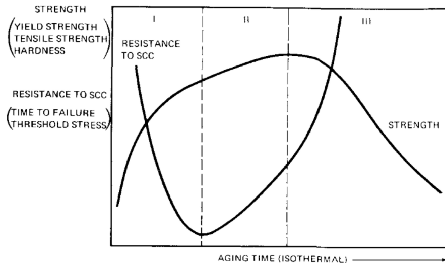
FIGURE 1.4: Variation of resistance to SCC and strength with aging time [12].
