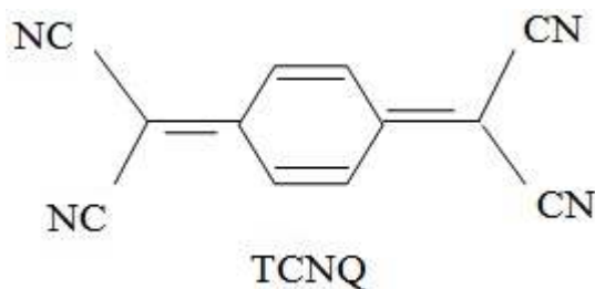
Fig. 2.4 Chemical structure of TCNQ
