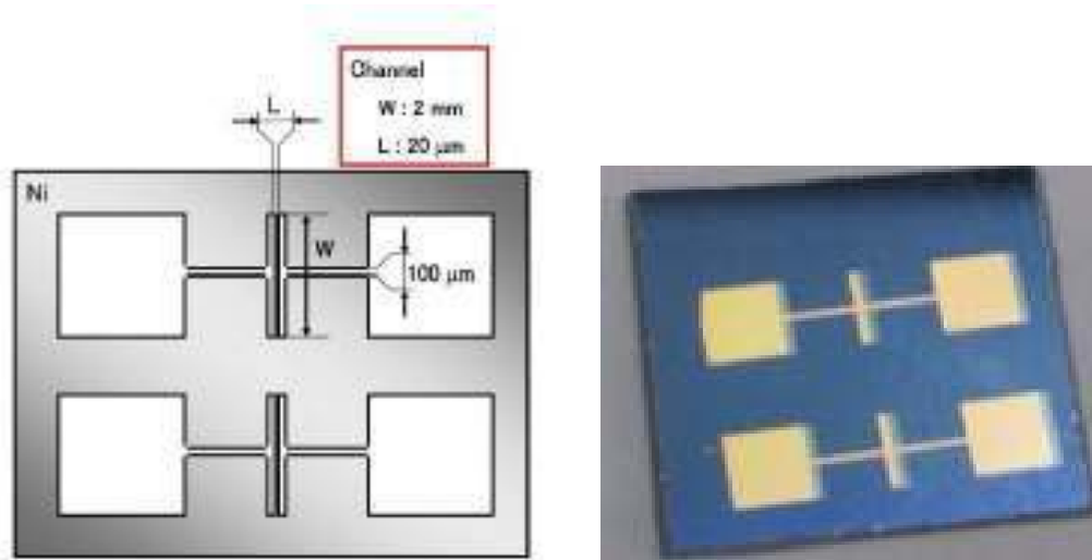
Fig. 2.10 (a) Schematic representation of the nickel mask used for the source and drain electrodes deposition [Arnaud et al. (2012)], (b) Image of the fabricated OFETs
