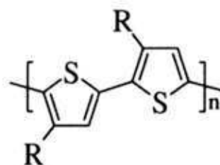
Fig. 2.1 Structure of P3HT
