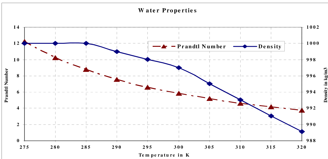
Fig. 5.10: Variation of Prandtl number and density at different temperatures.
