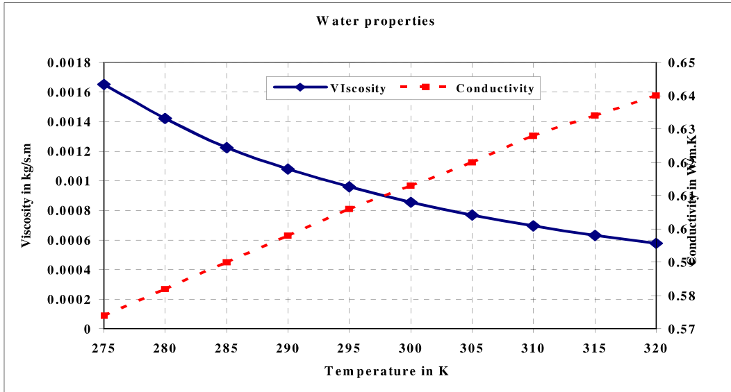
Fig. 5.9: Variation of water viscosity and conductivity at different temperatures.
