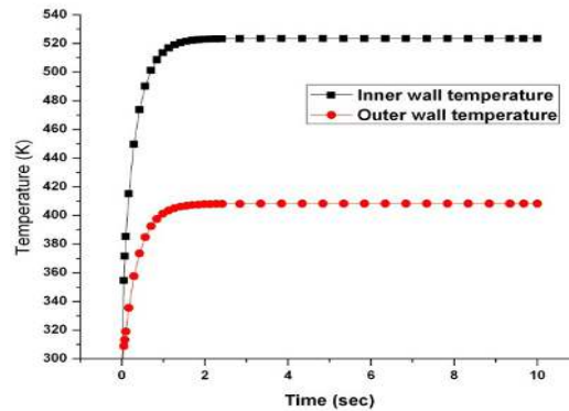
Fig. 5.16: Collector temperature versus time (axial grooves = 18, water temp 293°K, beam spread = 330mm, hydraulic dia = 4.5mm, water flow rate = 800L/m, power dissipation = 650kW).
