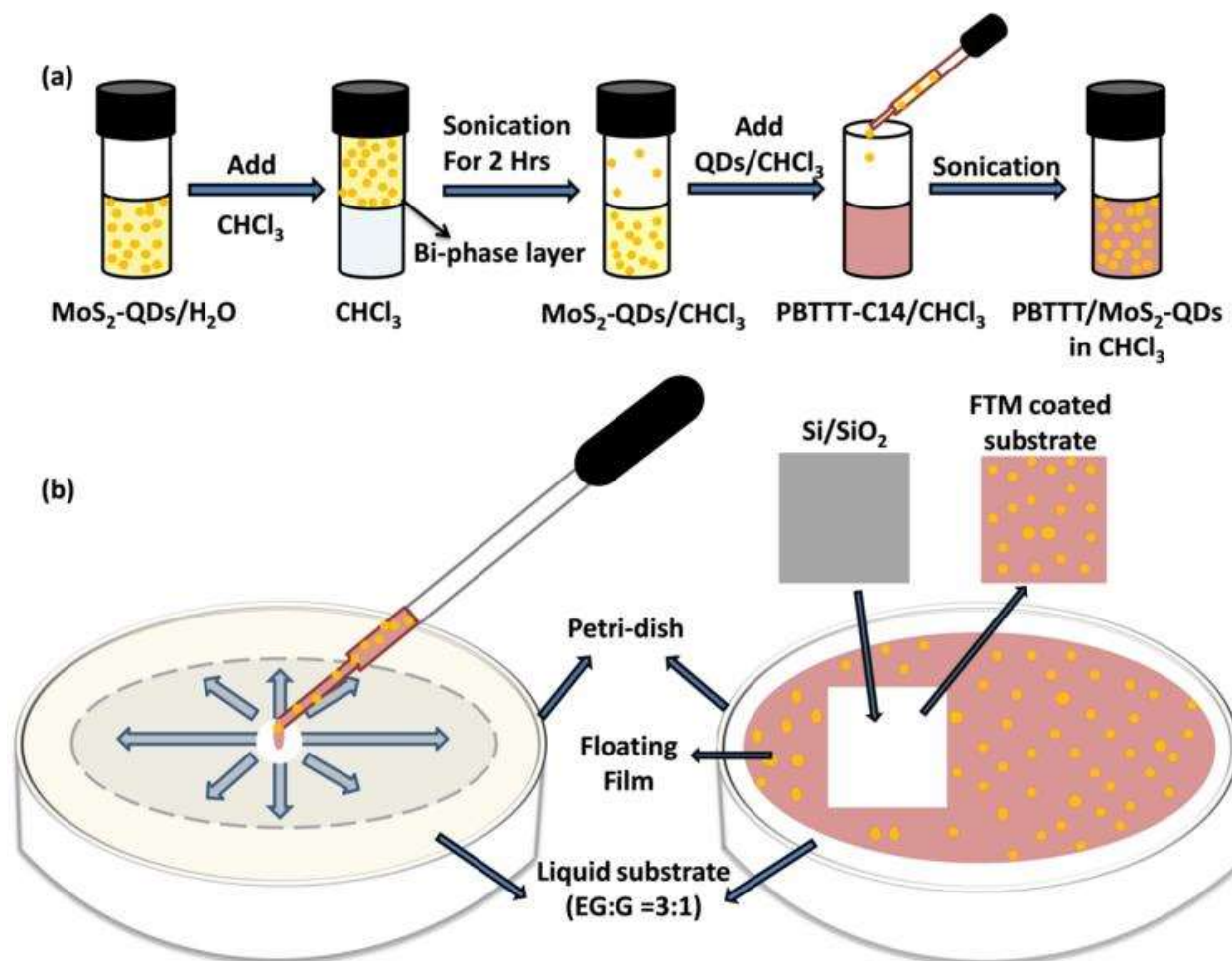
Fig. 3.2. Schematic illustration of (a) Phase transfer method to transfer \text{MoS}_2\text{-QDs} from water to chloroform; (b) FTM method for PBTTT-C14/ \text{MoS}_2\text{-QDs} based hybrid film spreading on the nonvolatile liquid substrate (EG:G = 3:1) and stamping of the film on the substrate.
