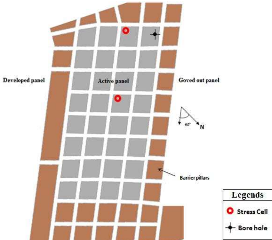
Fig. 4.10 Layout of the panel in 'Case B'
