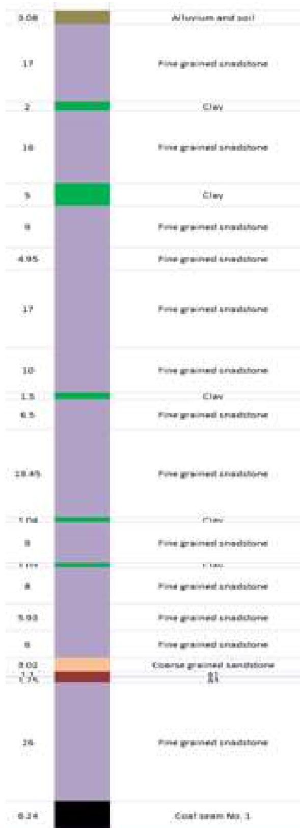
Fig. 4.1 Borehole log of the strata in 'Case A'
