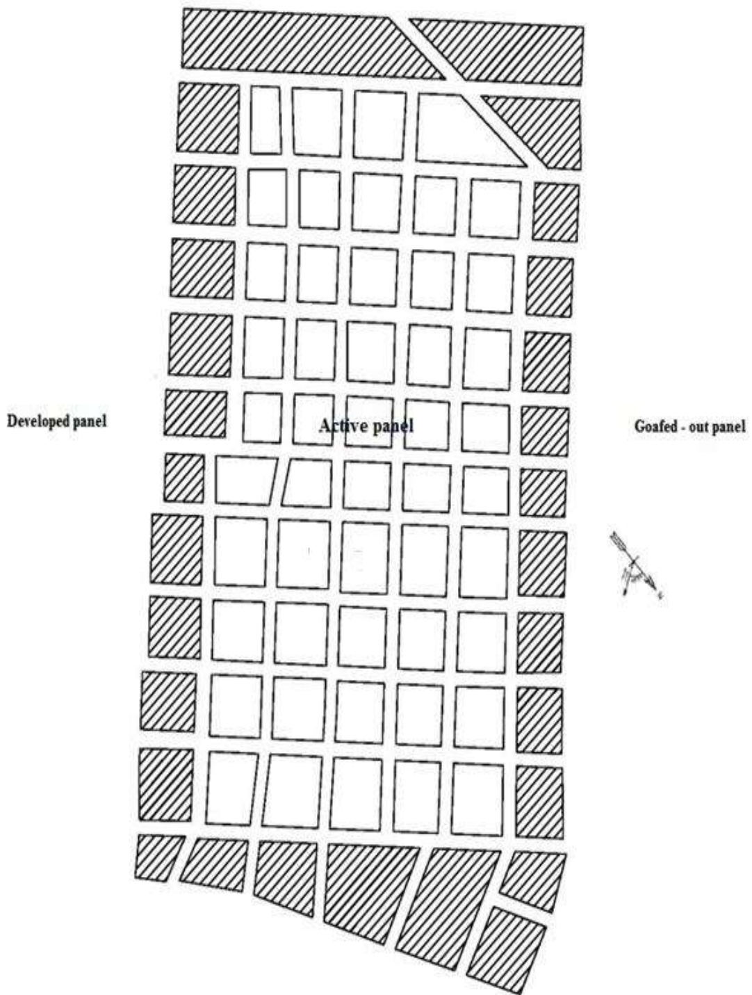
Fig. 4.2 Layout of the panel in 'Case A'
