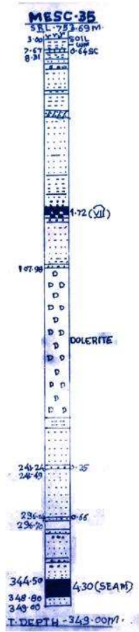
Fig. 4.16 Borehole of the strata in 'Case C'
