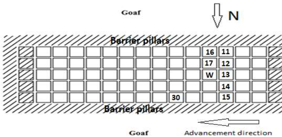
Fig. 4.17 Layout of the panel in 'Case C'
