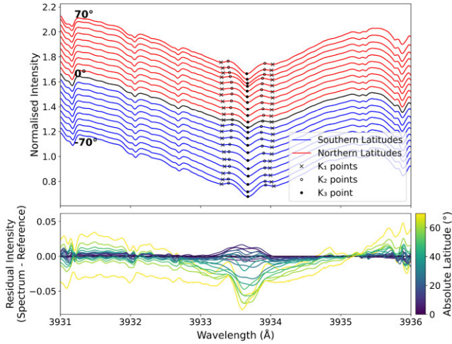
Figure 3. Top: LW Ca-K line profiles from our observations. Starting from -70^\circ , the profiles are successively offset vertically by 0.05 units for visual clarity. Bottom: residual intensity plot of the profiles taking the profile at the equator as the reference.
