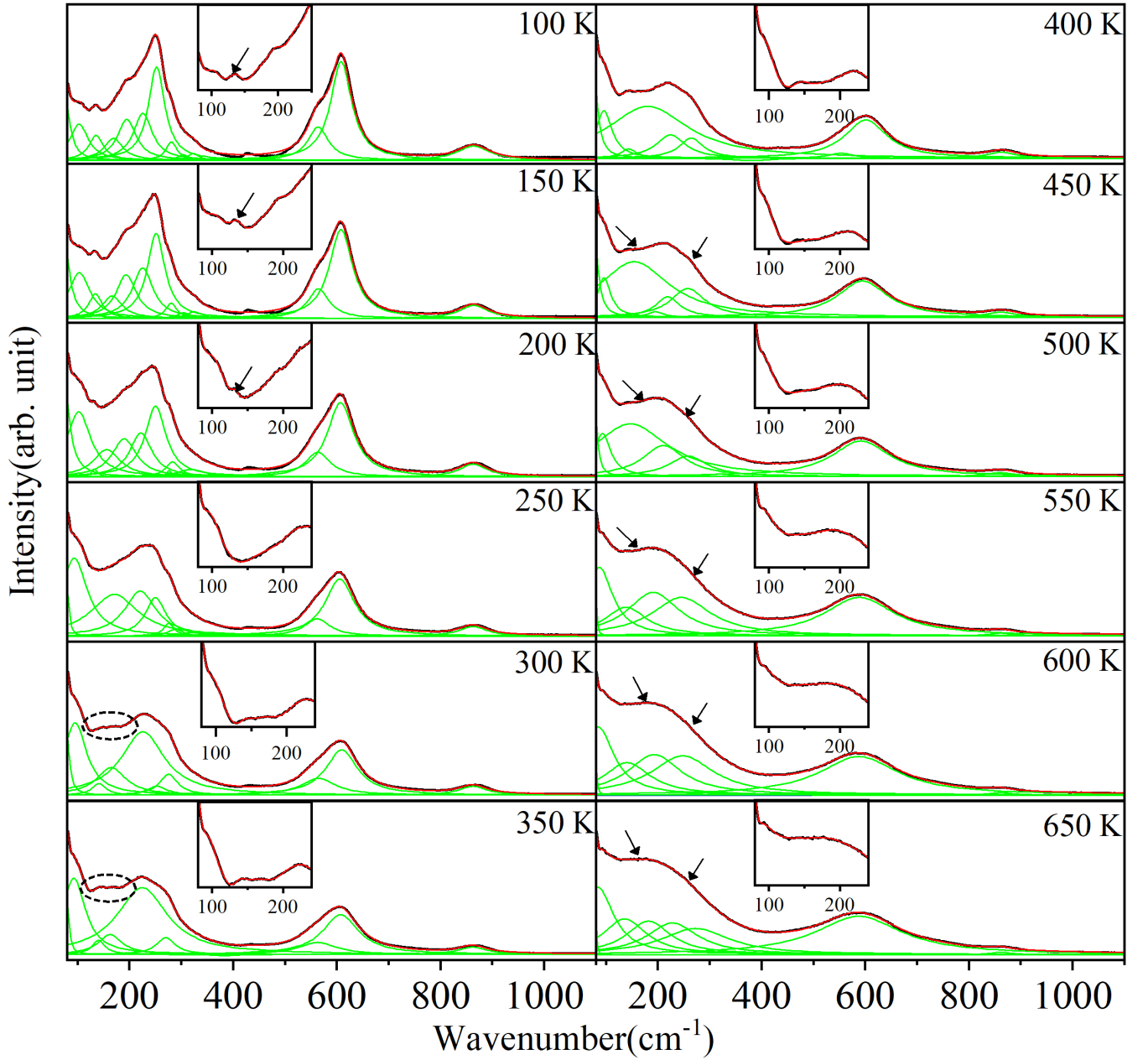
FIG. 4. Raman spectra of NN-10BCT at different temperatures in the range of 100-650 K. The Raman spectra have been taken during the heating cycle using the protocol described in the experimental section. All the Raman spectra have been deconvoluted using a suitable number of Lorentz peaks.
