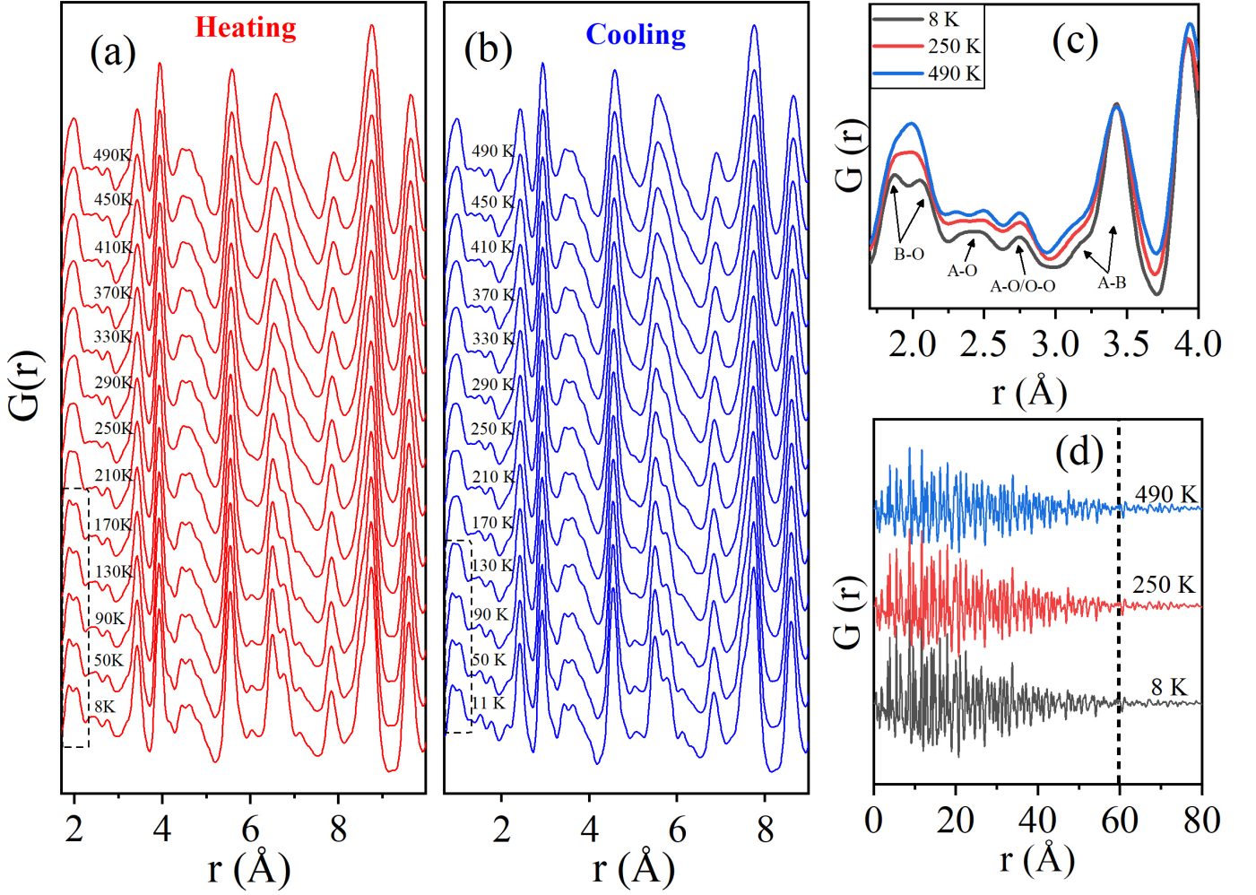
FIG. 6. Experimental Variable temperature G(r) for r \approx 1-10 Å for 0.9\text{NaNbO}_3-0.1\text{Ba}_{0.9}\text{Ca}_{0.1}\text{TiO}_3 ceramic powders in (a) Heating (b) Cooling modes, showing the evolution of short-range structures (c) Experimental G(r) within \approx 4 Å, showing the nearest neighbour pairwise atomic correlations. (d) G(r) depicting the length of structural coherence at some representative temperatures
