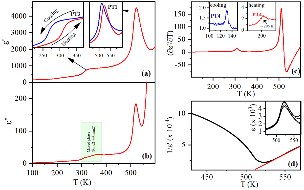
FIG. 1. Temperature dependent (a) real and (b) imaginary part of dielectric permittivity in a wide temperature range of 100 K-600 K. (c) Derivative of the real part of dielectric permittivity with respect to temperature marking the weak phase transition around 200 K and 130 K during the heating and cooling cycle respectively. (d) The inverse of dielectric permittivity is plotted against the temperature. The inset shows the frequency-independent dielectric maxima, which is a feature of classical ferroelectric material.
