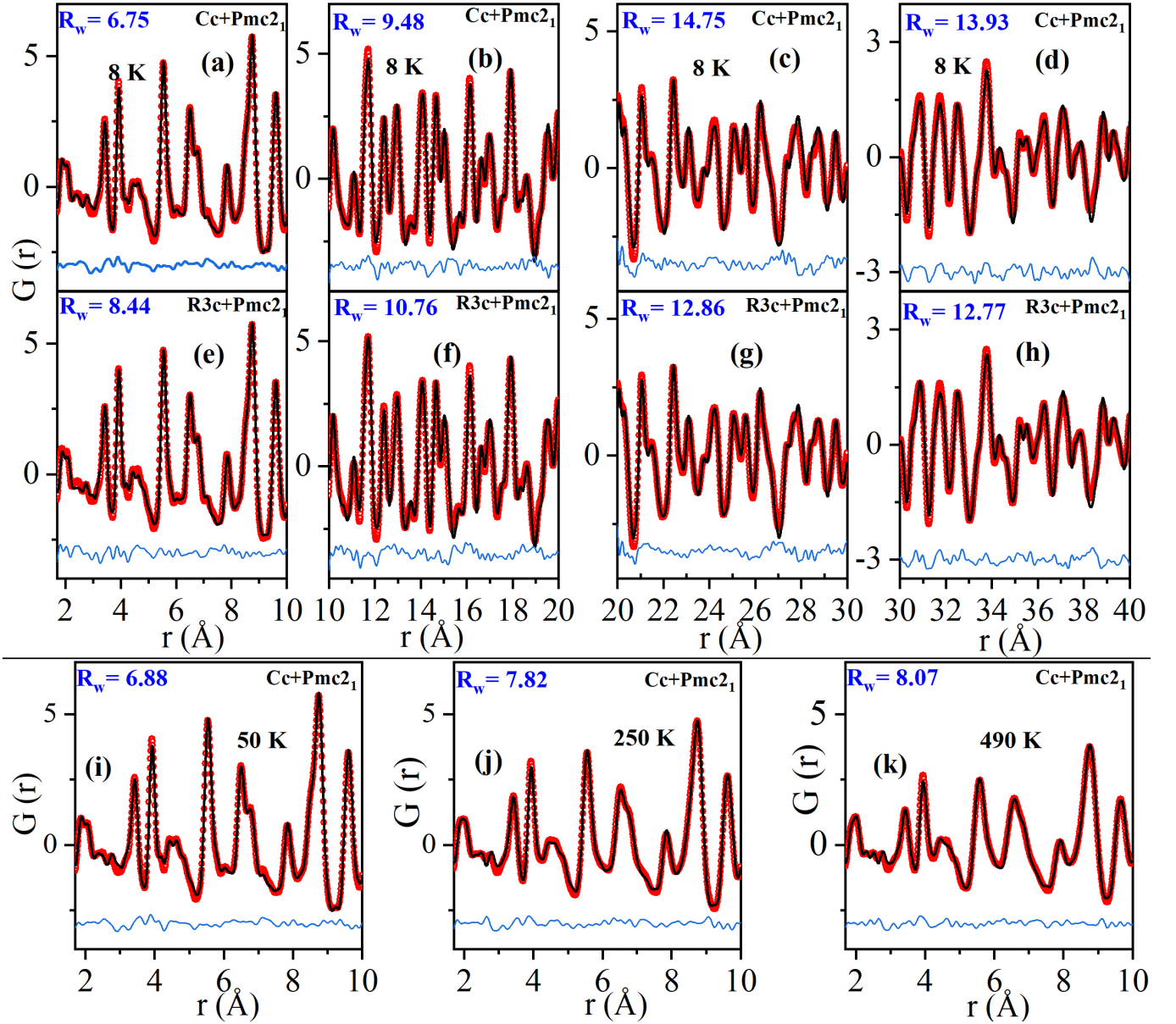
FIG. 7. Refinement of PDF profile for different length scale at 8 K using (a)-(d) Cc+Pmc2 1 model & (e)-(h) R3c+Pmc2 1 models. PDF refinement with Cc+Pmc2 1 model for 1.7 \leq r \leq 10 Å at different temperatures viz., 50K, 250 K, and 490 K have been shown in (i), (j) and (k), respectively.
