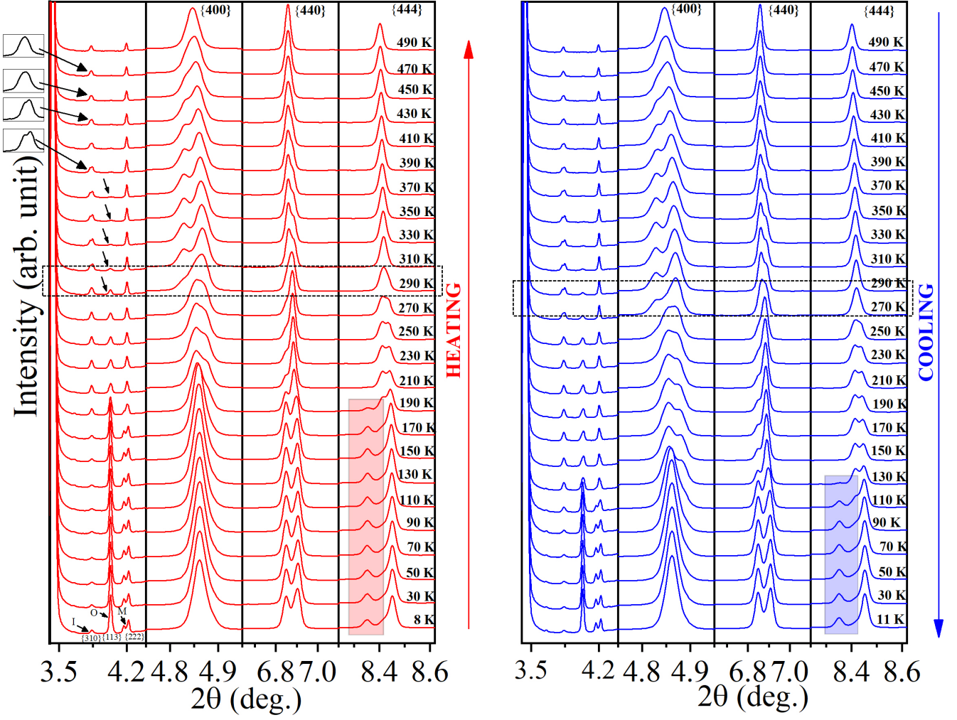
FIG. 2. Evolution of Main perovskite reflections viz., \{400\}_{\text{dpc}} , \{440\}_{\text{dpc}} and \{444\}_{\text{dpc}} as well as superlattice reflections in (a) Heating (b) Cooling cycle. The shaded rectangle shows the appearance of a new peak beside the \{444\}_{\text{dpc}} reflection around 190 K and 130 K during the heating and cooling cycles, respectively. The dashed rectangle shows the changes in the main perovskite reflections around room temperature.
