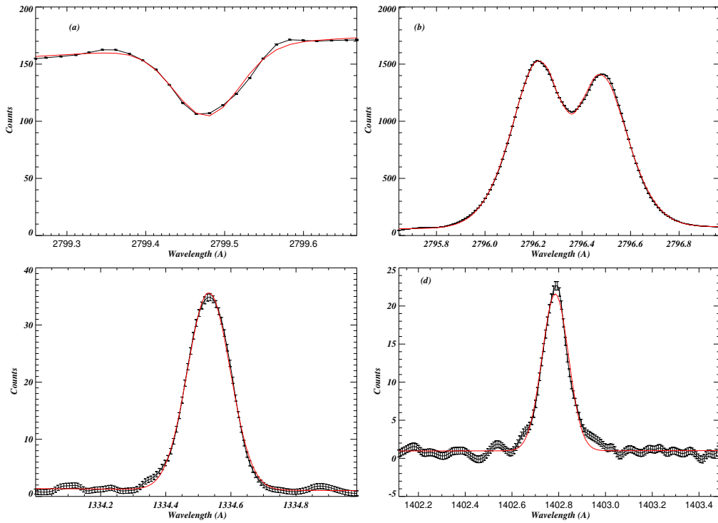
Figure 3.8: Spectral fitting of (a) Ni I ( 2799.47 \text{ \AA} ), (b) Mg II k ( 2796.2 \text{ \AA} ), (c) C II ( 1354.53 \text{ \AA} ), and (d) Si IV ( 1402.77 \text{ \AA} ) lines for box labelled as B3 in the left panel Fig. 3.10 for Dataset 3.
