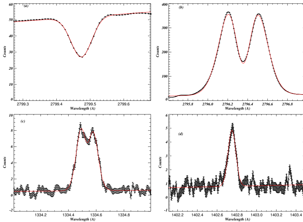
Figure 3.5: Spectral fitting of (a) Ni I (2799.47 Å), (b) Mg II k (2796.2 Å), (c) C II (1354.53 Å), and (d) Si IV (1402.77 Å) lines for averaged profile over the box labelled as B4 shown in the left panel of Fig. 3.7 corresponding to Dataset 2.
