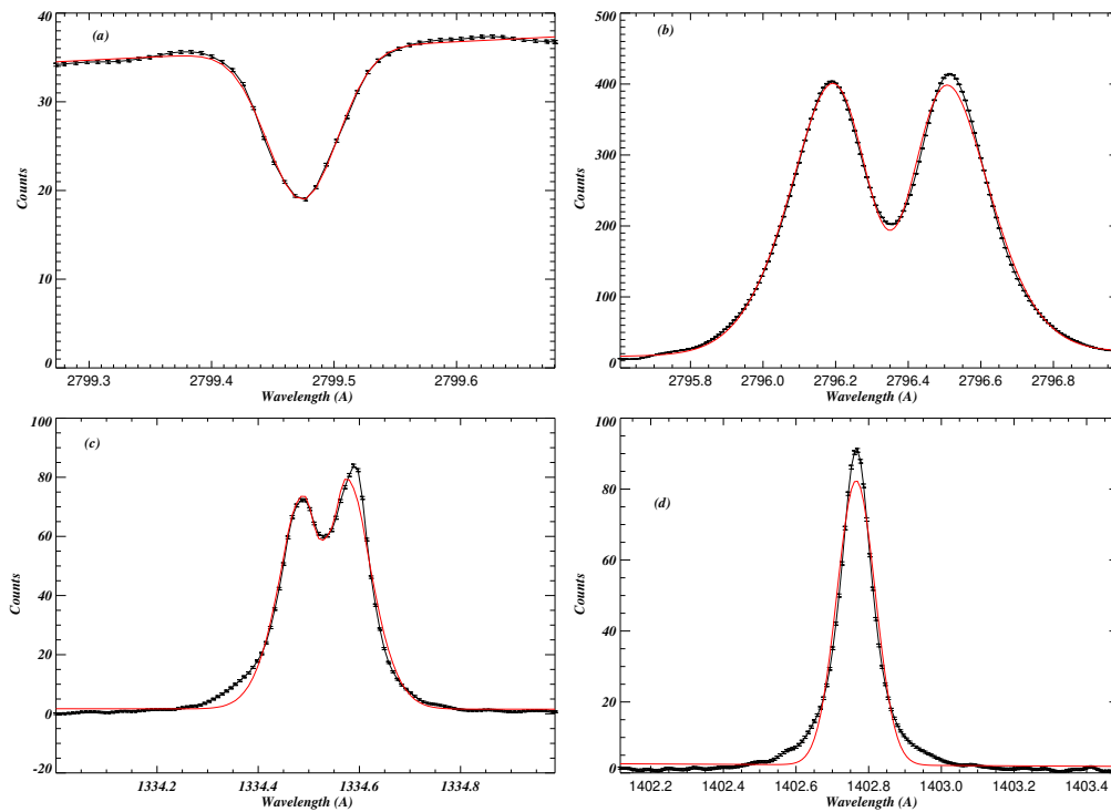
Figure 3.2: Spectral fitting of (a) Ni I (2799.47 Å), (b) Mg II k (2796.2 Å), (c) C II (1354.53 Å), and (d) Si IV (1402.77 Å) lines for averaged profile over the box labelled as B5 shown in the Si IV left panel of Fig. 3.4 corresponding to Dataset 1.
