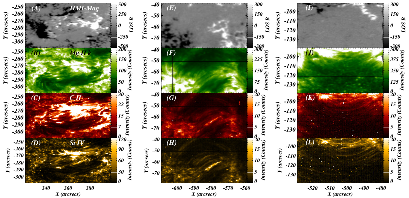
Figure 3.1: The region of interest displaying the cool loop system in different spectral lines: Mg II k (2796.20 Å), C II (1334.53 Å), and Si IV (1402.77 Å) along with the underlying magnetic polarities indicated by HMI LOS magnetogram are shown for three different datasets. The left column corresponds to Dataset 1 observed on 27th December 2013 targeting AR 11934. The middle column indicates Dataset 2 observed on 10th December 2015 targeting AR 12465. The right column shows the Dataset 3 observed on 29th March 2017 targeting AR 12645.
