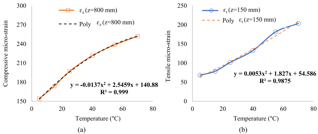
Fig. 21. Effect of temperature on (a) \epsilon_z and (b) \epsilon_t under LVE simulations.
