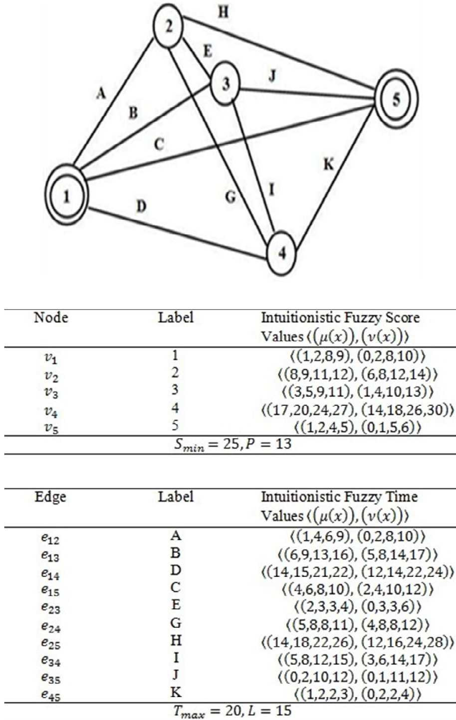
Fig. 3.7: The input graph with N = 5, v_1 = 1, v_N = 5 and the time and score values associated with each edge and vertex respectively
