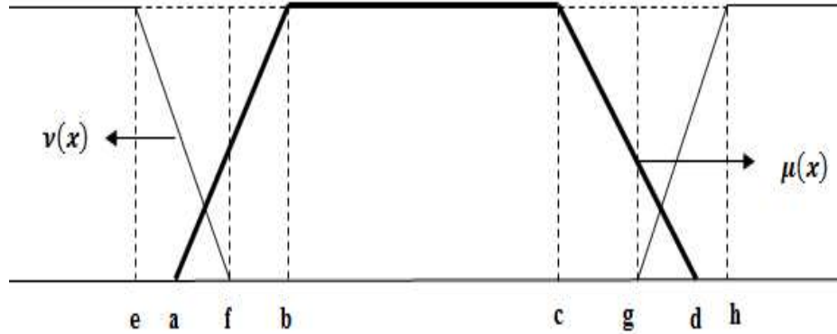
Fig. 3.1: Trapezoidal intuitionistic fuzzy number (TIFN)
