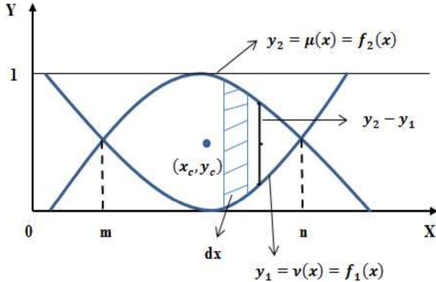
Fig. 3.5: Centroid method of ranking for QGIFN
