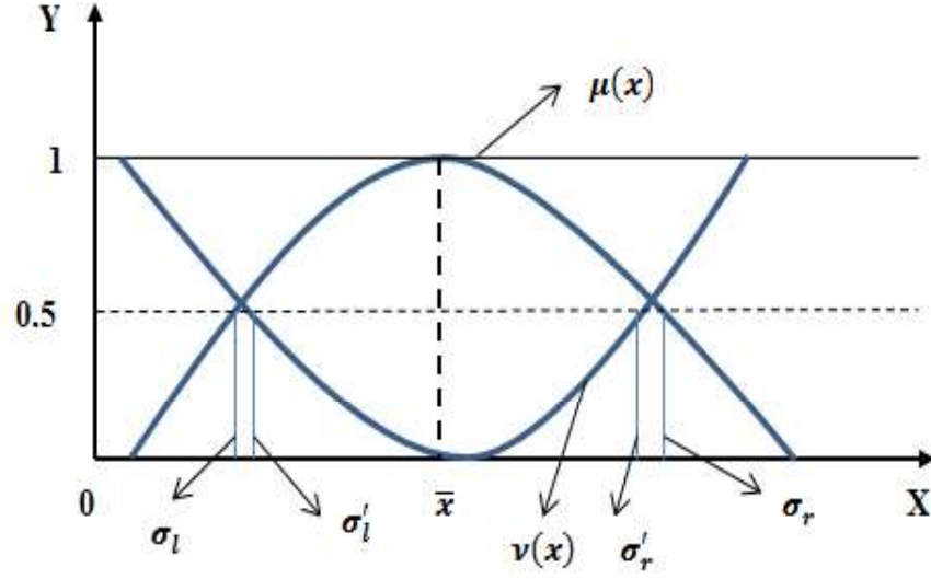
Fig. 3.4: Quasi-Gaussian Intuitionistic Fuzzy Number
