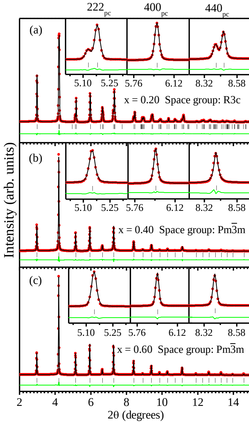
Figure 3.4: Rietveld refinement using synchrotron x-ray diffractogram of (1-x)\text{BiFeO}_3-x\text{BaTiO}_3 powders for representative compositions x = 0.20 , 0.40 , 0.60 using (a) Rhombohedral R\bar{3}c space group (b) Cubic Pm\bar{3}m space group and (c) Cubic Pm\bar{3}m space group. Inset depicts the fits for the pseudocubic reflections 222_{pc} , 400_{pc} and 440_{pc} .
