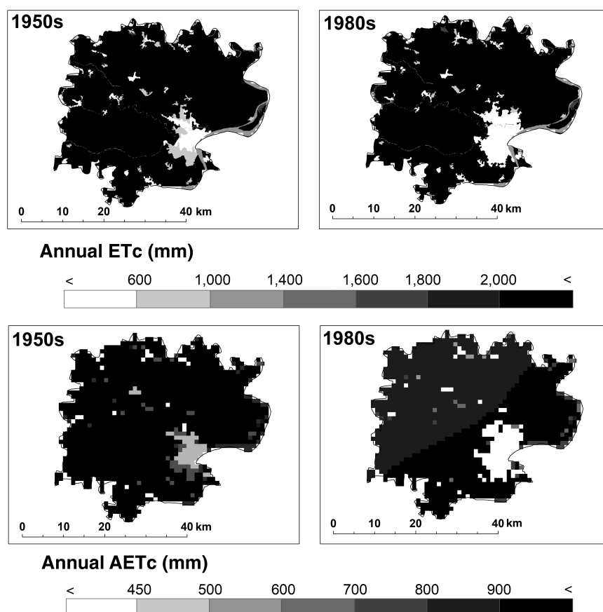
FIGURE 5 Spatial distribution of annual crop evapotranspiration ( ET_c ) and actual crop evapotranspiration ( AET_c ) in Varanasi district: (a) annual ET_c related to the 1950s; (b) annual ET_c related to the 1980s; (c) annual AET_c related to the 1950s; and (d) annual AET_c related to the 1980s
