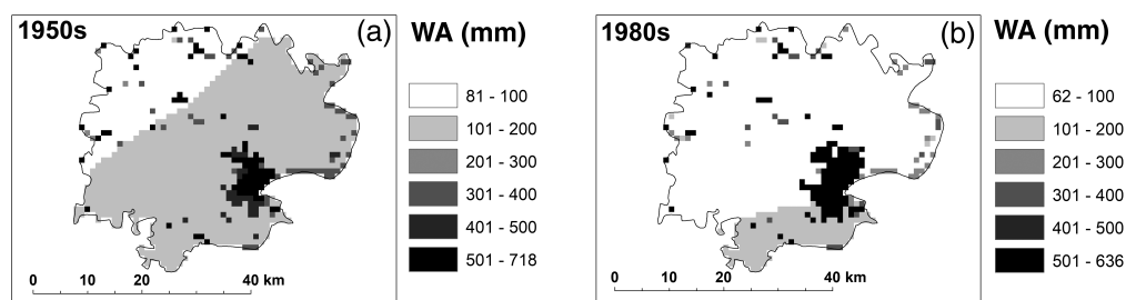
FIGURE 6 Spatial distribution of annual water availability (WA) in Varanasi district: (a) annual WA related to the 1950s; and (b) annual WA related to the 1980s
