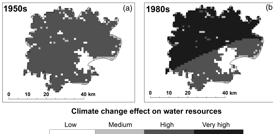
FIGURE 8 Climate effect assessment on water resources in Varanasi district: (a) spatial distribution of climate effect during the 1950s; and (b) spatial distribution of climate effect during the 1980s
