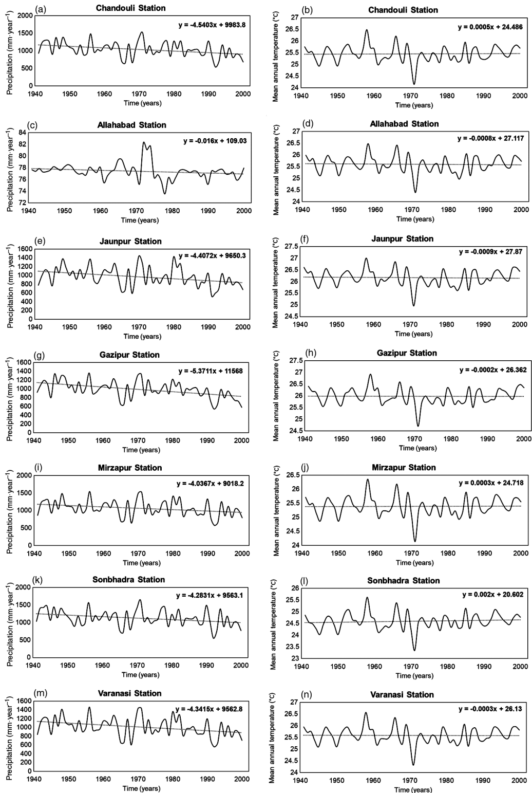
FIGURE 4 Annual trends of precipitation and temperature at meteorological stations during the period 1941–2000
