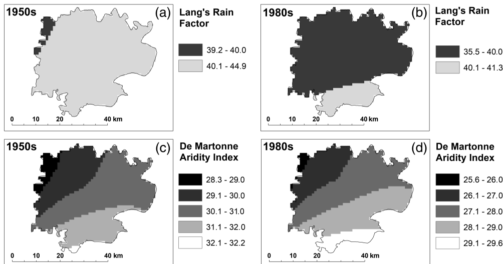
FIGURE 7 Spatial distribution of the Lang's rain factor and De Martonne's aridity index: (a) Lang's rain factor related to the 1950s; (b) Lang's rain factor related to the 1980s; (c) De Martonne's aridity index related to the 1950s; and (d) De Martonne's aridity index related to the 1980s
