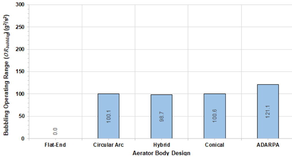
FIG. 14: Effect of aerator body design on bubbly flow operating range
