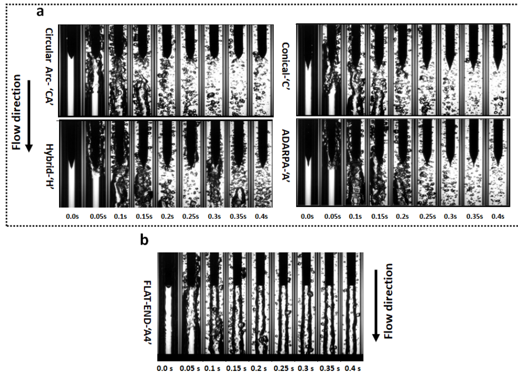
FIG. 11: Ability of aerator tip to passively bleed mixing chamber of ambient gas: (a) liquid flow range: 75–289 g/s, 0% ALR; (b) operating pressure: 5 bar
