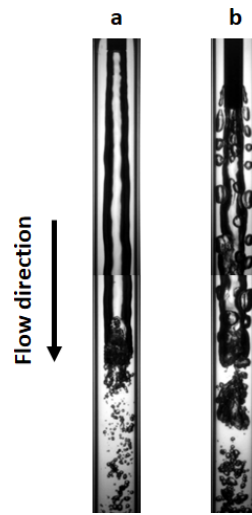
FIG. 8: Examples of gas void shearing: (a) liquid Baker parameter: 742 \text{ kg/m}^2\text{s} , 0.002% ALR; (b) liquid Baker parameter: 605 \text{ kg/m}^2\text{s} , 0.41% ALR
