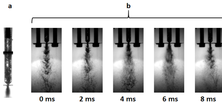
FIG. 10: Atomization of gas void disintegrated slug flow: (a) internal flow; (b) near-nozzle. Images are acquired by high-speed shadowgraphy.
