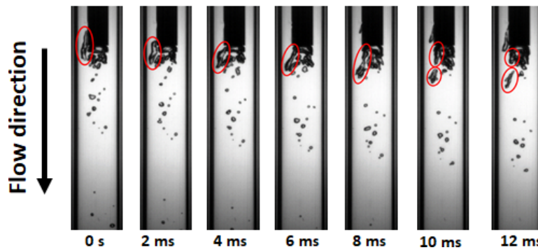
FIG. 7: Observation of gas entity entrapment in aerator wake from bled start-up (ALR: 0.003%)
