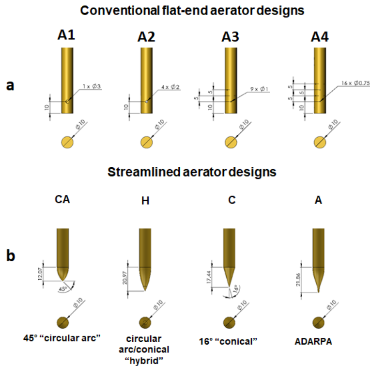
FIG. 4: (a) Conventional flat-end aerator designs employed in the present study (dimensions in mm) (b) Streamlined aerator body designs (dimensions in mm): CA, 45° "circular arc" (Silhan and Cubbage, 1957); H, circular arc/conical "hybrid" (Mair, 1969); C, 16° "conical" (Silhan and Cubbage, 1957); A, "ADARPA" (Groves et al., 1989)
