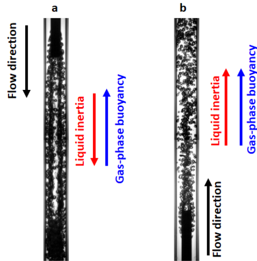
FIG. 6: Example observation of effect of orientation at comparable ALR and fully open discharge nozzle setting (i.e., equivalent exit orifice diameter) for A3 configuration: (a) vertically downwards, 0.13% ALR; (b) vertically upwards, 0.12% ALR
