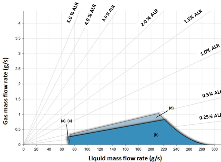
FIG. 13: Effect of aerator body design on bubbly flow operating range: (a) CA, circular arc; (b) H, hybrid; (c) C, conical; (d) A, ADARPA
