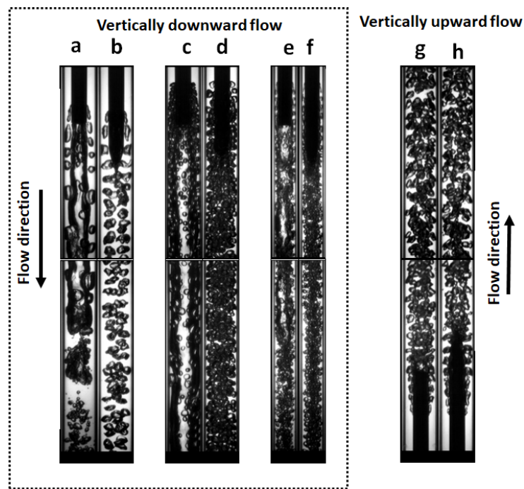
FIG. 12: Comparison of flat-end and ADARPA aerator body designs for equivalent operating conditions: (a) flat-end: liquid Baker parameter: 808.9 \text{ kg/m}^2\text{s} , 0.13% ALR; (b) ADARPA: liquid Baker parameter: 802.5 \text{ kg/m}^2\text{s} , 0.12% ALR; (c) flat-end: liquid Baker parameter: 257.9 \text{ kg/m}^2\text{s} , 0.26% ALR; (d) ADARPA: liquid Baker parameter: 261.1 \text{ kg/m}^2\text{s} , 0.25% ALR; (e) flat-end: liquid Baker parameter: 433.1 \text{ kg/m}^2\text{s} , 0.25% ALR; (f) ADARPA: liquid Baker parameter: 433 \text{ kg/m}^2\text{s} , 0.26% ALR; (g) flat-end: liquid Baker parameter: 745 \text{ kg/m}^2\text{s} , 0.25% ALR; (h) ADARPA: liquid Baker parameter: 748.4 \text{ kg/m}^2\text{s} , 0.25% ALR
