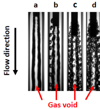
FIG. 5: Example observations of gas void formation in aerator wake for different aerator configurations: (a) configuration: A1; ALR: 0.02%; (b) configuration: A2; ALR: 0.03%; (c) configuration: A4; ALR: 0.13%; (d) configuration: A4; ALR: 0.25%
