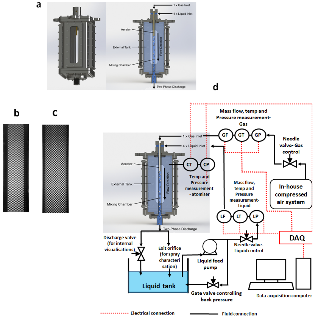
FIG. 2: Experimental test facility and fluid flow circuit employed in the present effervescent atomizer study. (a) Effervescent atomizer with aerator and mixing chamber; (b) image distortion through a cylindrical mixing chamber without refraction minimization; (c) image with water tunnel; (d) fluid supply lines and its controllers.
