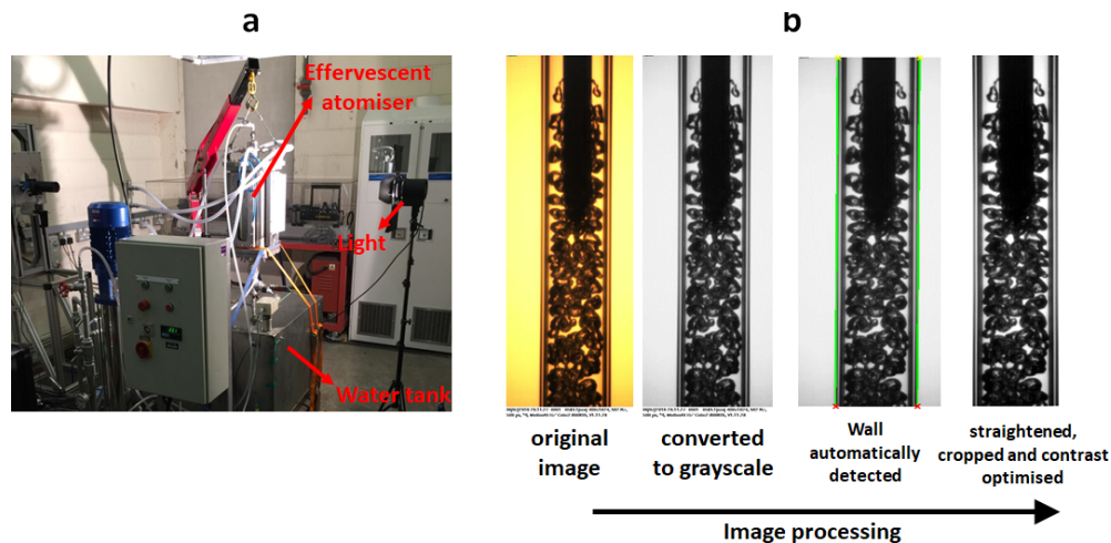
FIG. 3: (a) High speed shadowgraphy set up. (b) Sequence of image processing applied to internal flow visualization images obtained from high speed shadowgraphy.
