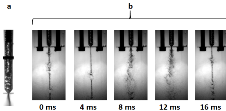
FIG. 9: Atomization of gas void disintegrated polydispersed bubbles (0.12% ALR): (a) internal flow and (b) near-nozzle. Images are acquired by high-speed shadowgraphy.
