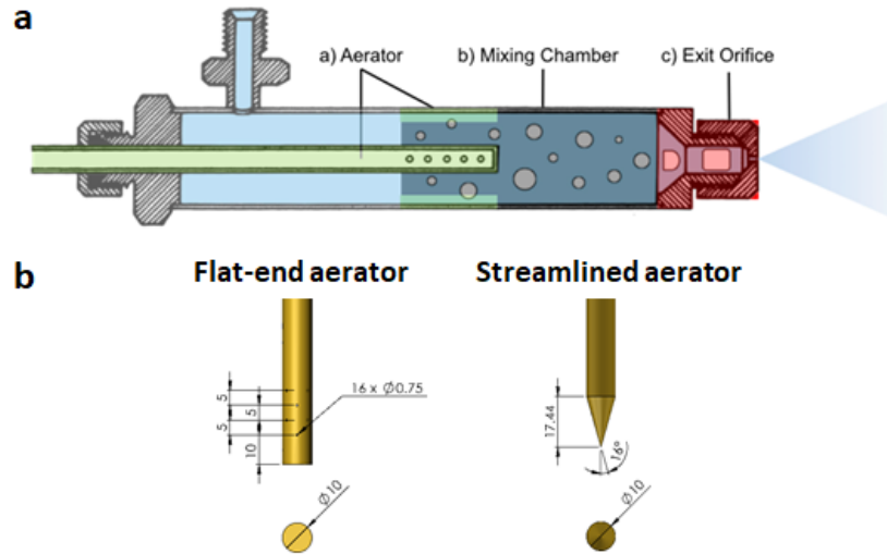
FIG. 1: (a) Effervescent atomizer common components. (b) Aerator body designs.
