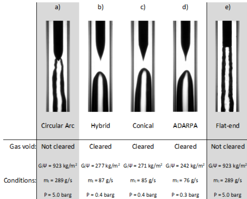
FIG. 15: Ability of aerator tips to remove established gas void from wake
